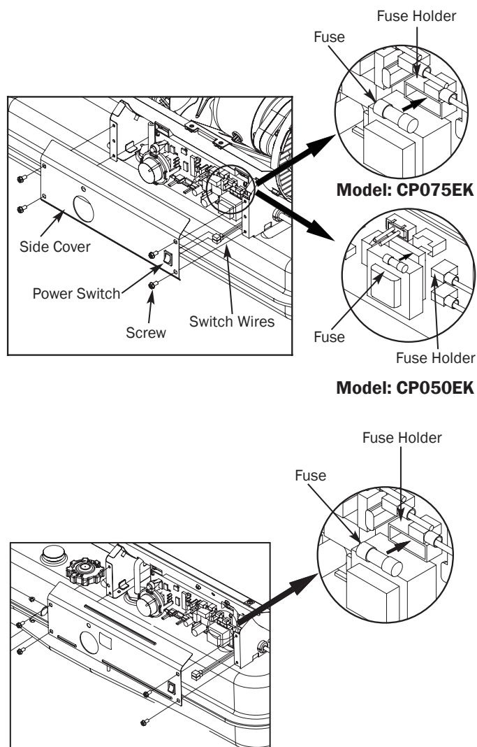
Figure 23 – Replacing Fuse
