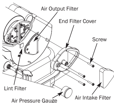
Figure 11 - Filter Assembly
