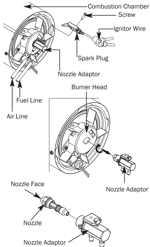
Figure 16 – Nozzle Replacement For Models CP050EK-CP175FK
