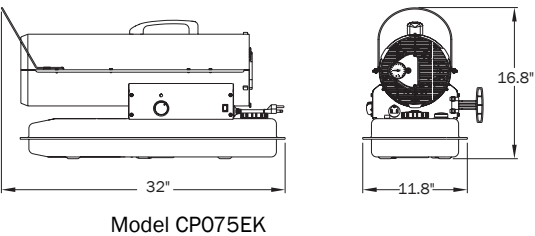
Figure 1.1 - Heater Dimensions
