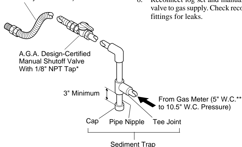
Figure 6 - Gas Connection
