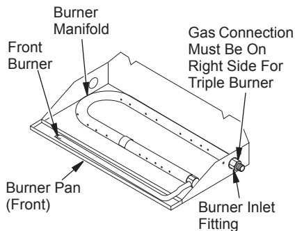
TRIPLE-BURNER
