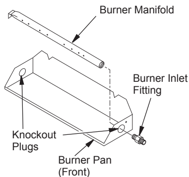
SINGLE-BURNER
