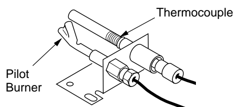
Figure 20 - Thermocouple and Pilot
