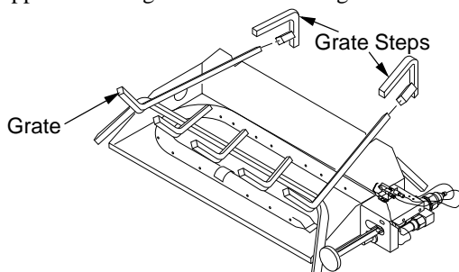
Figure 16 - Installing Grate (Pan Material Not Shown)
