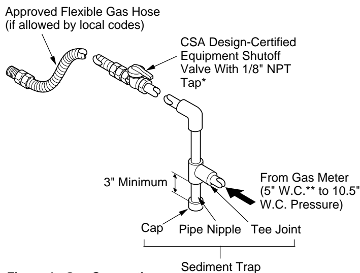
Figure 4 - Gas Connection
