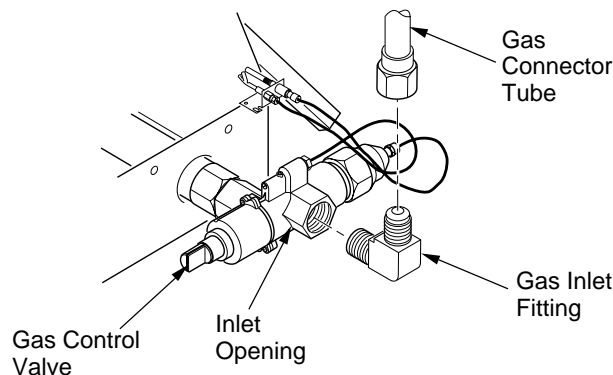
Figure 11 - Installing Inlet Fitting and Gas Connector Tube
