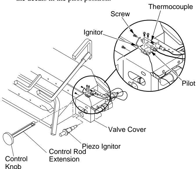
Figure 12 - Installing Cover, Control Knob, and Piezo Ignitor
