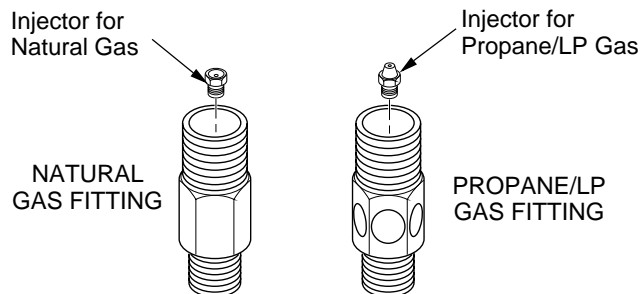
Figure 13 - Burner Inlet Fittings with Injectors
