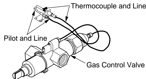
Figure 10 - Gas Control Valve with Thermocouple and Pilot
