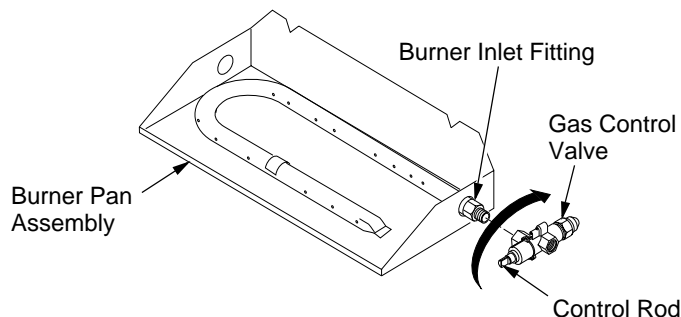
Figure 9 - Installing Gas Control Valve
