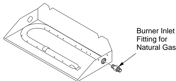
Figure 14 - Remove Burner Inlet Fitting
