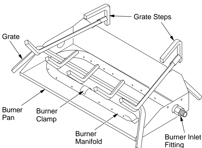
Figure 1 - Product Identification (Dual Burner Shown)
