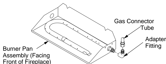
Figure 8 - Connecting Gas to Appliance
