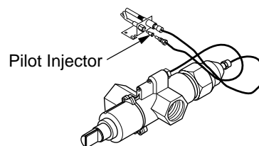
Figure 15 - Installing Propane/LP Pilot Orifice
