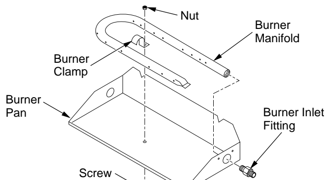
Figure 7 - Installing Burner
