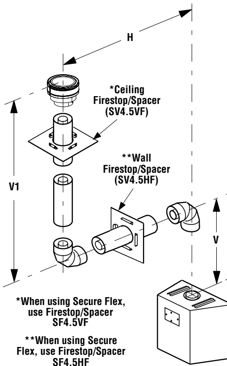
Figure 32 - Top Vent - TWO 90 DEGREE ELBOWS
