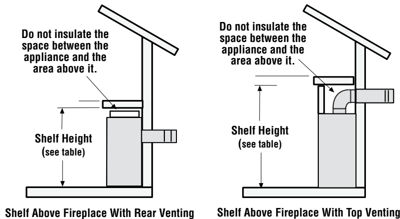
Figure 8 - Shelf Height Minimum Clearances With Top Venting
