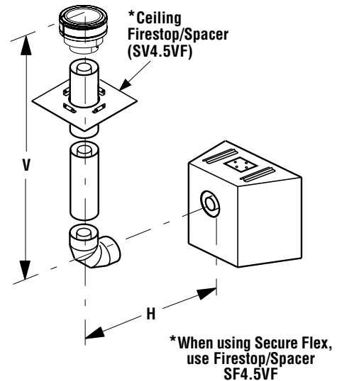
Figure 31 - Rear Vent - ONE 90 DEGREE ELBOW
