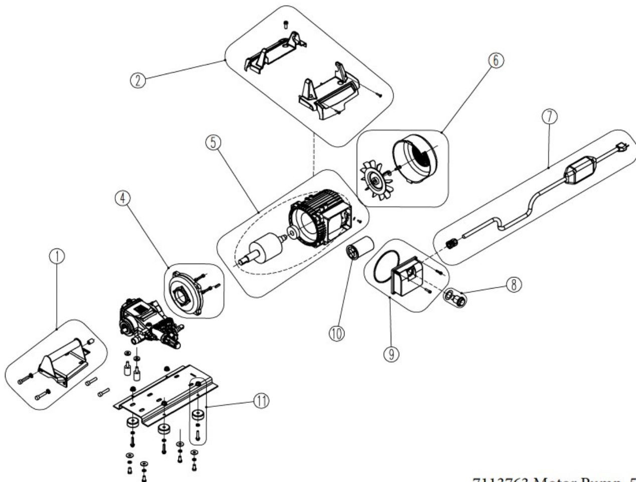
7113763 Motor Pump 53009.1 REV A
