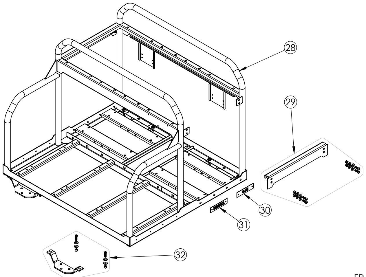
FRAME
