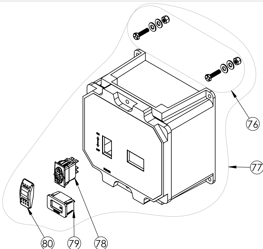
ELECTRICAL BOX
