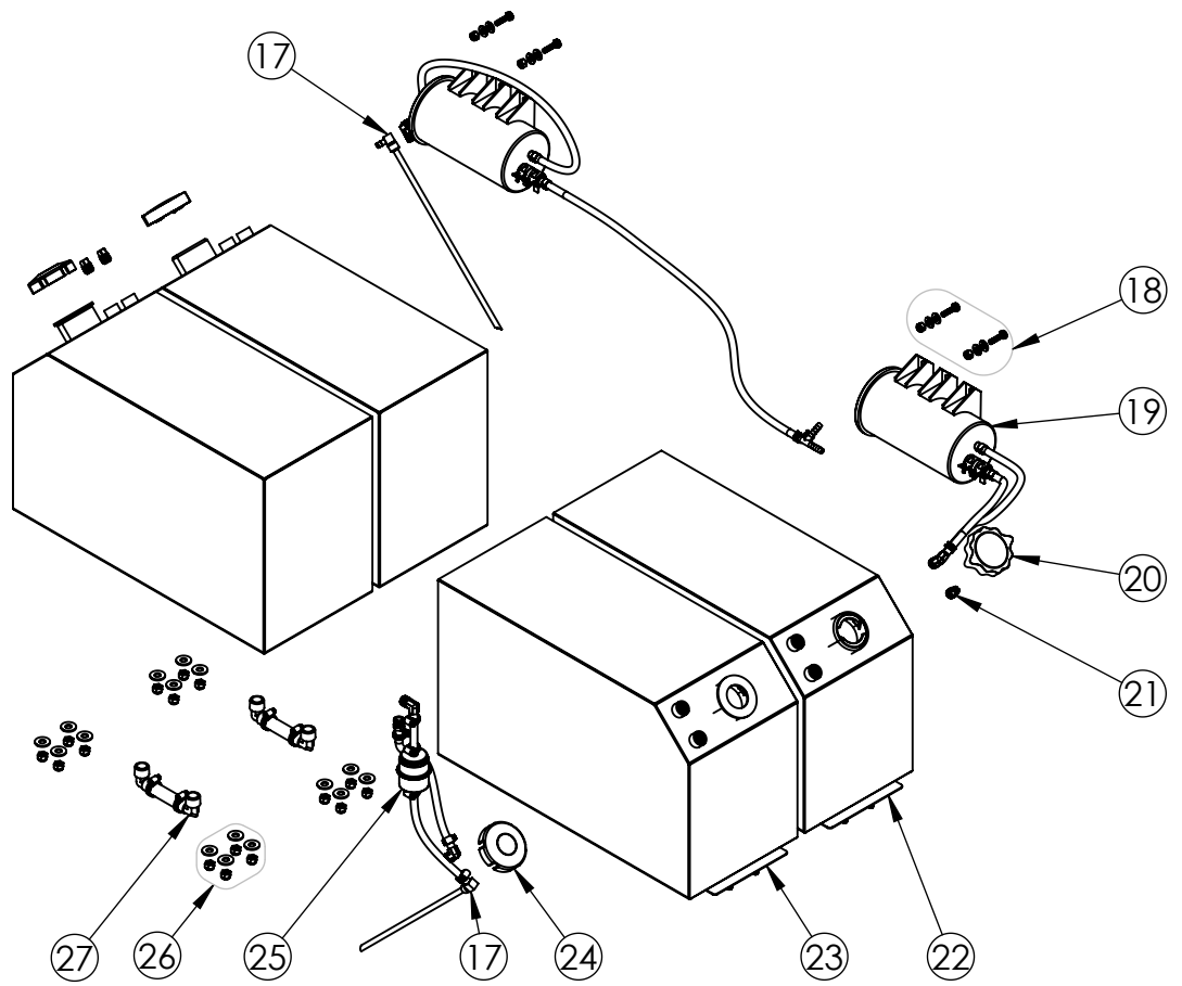
FUEL SYSTEM
