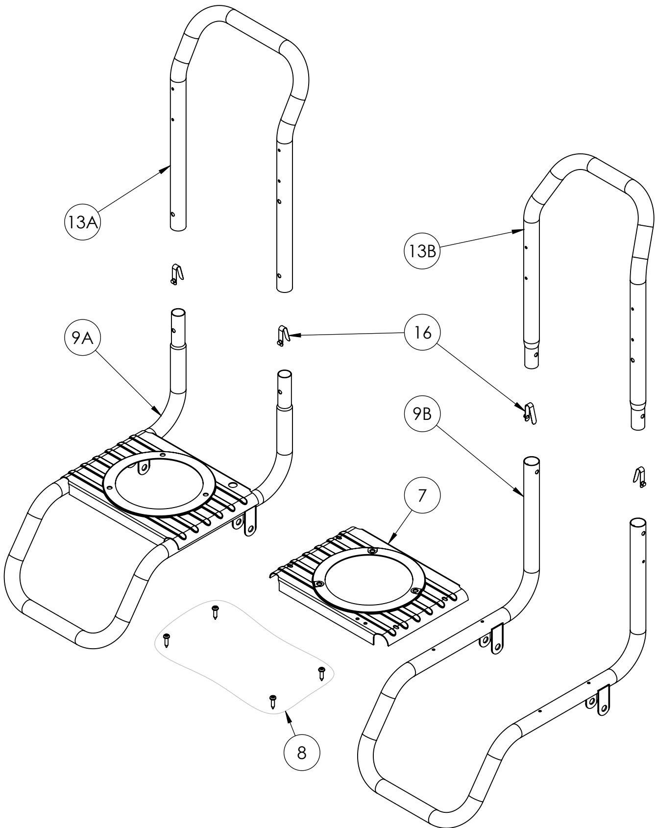
OLD WELDED FRAME
