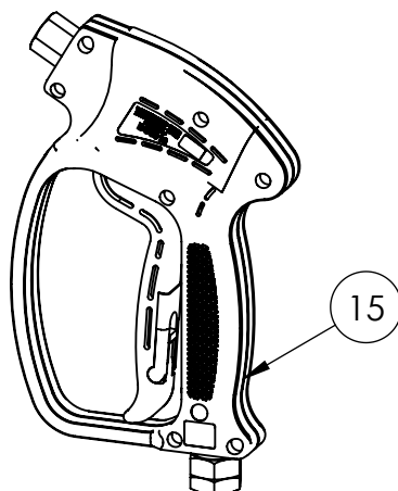
TRIGGER SPRAY GUN 4000PSI @ 8GPM PART NO. 7101787
