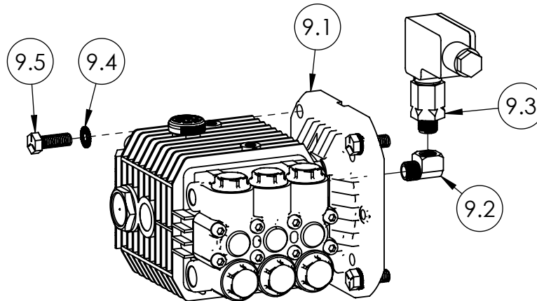
GP PUMP, SVC ASSY DD1003 PART NO. 7107041
