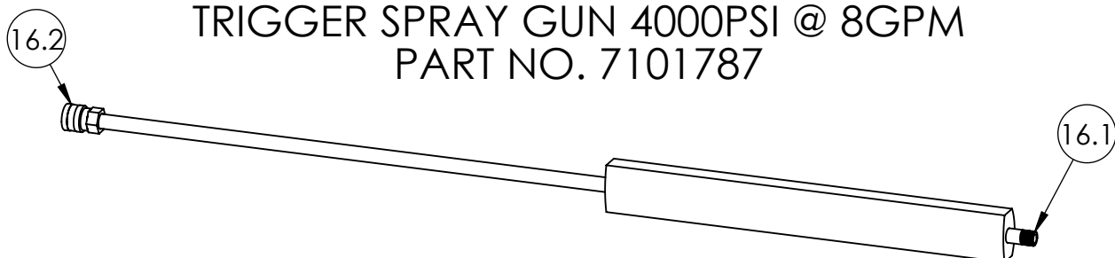
LANCE, 36" INSULATED PART NO. 7100550
