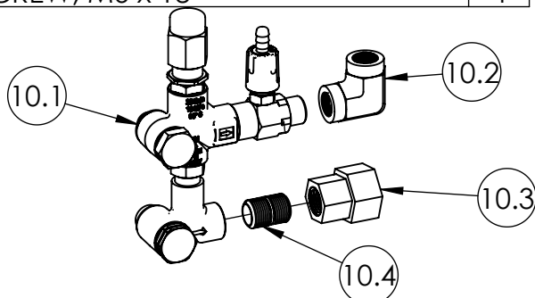
UNLOADER, SVC ASSY DD1003 PART NO. 7107042
