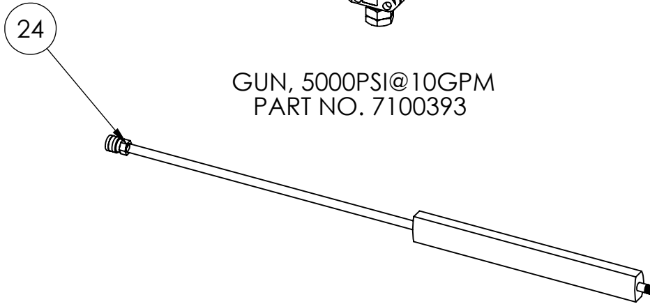
LANCE, 48IN 1/4MPT QC(F) PART NO. 7100551
