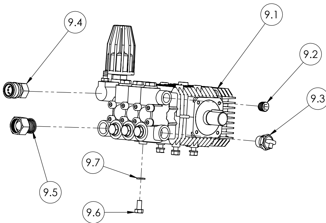
PUMP ASSEMBLY PART NO. 7106189
