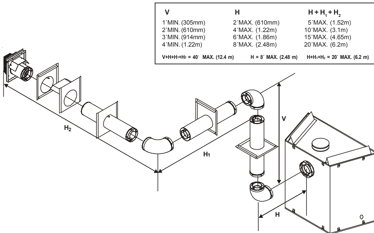
Figure 16. Venting with three 90° elbows
