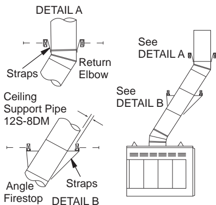
Figure 13 - Chimney Supports
