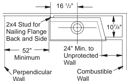
Figure 3 - Corner Installation
