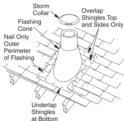
Figure 19 - Flashing Installation
