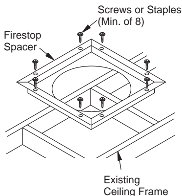
Figure 15 - Firestop Spacer with Attic Space Above Ceiling
