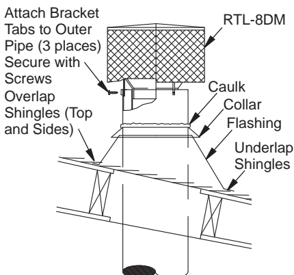
Figure 21 - Terminations
