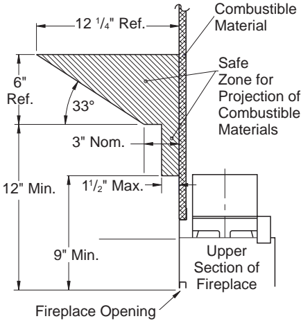
Figure 6 - Mantel Clearances
