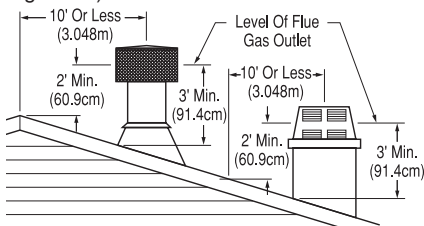
Figure 23 - 10 Foot Rule
