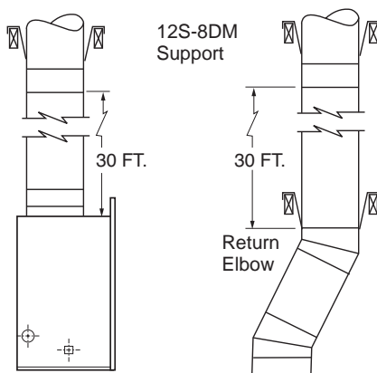
Figure 16 - Support Sections
