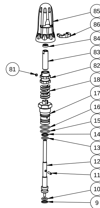
73 PART NO. 7108745 UNLOADER KIT
