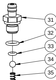
72 PART NO. 7104228 SOAP INJECTOR KIT
