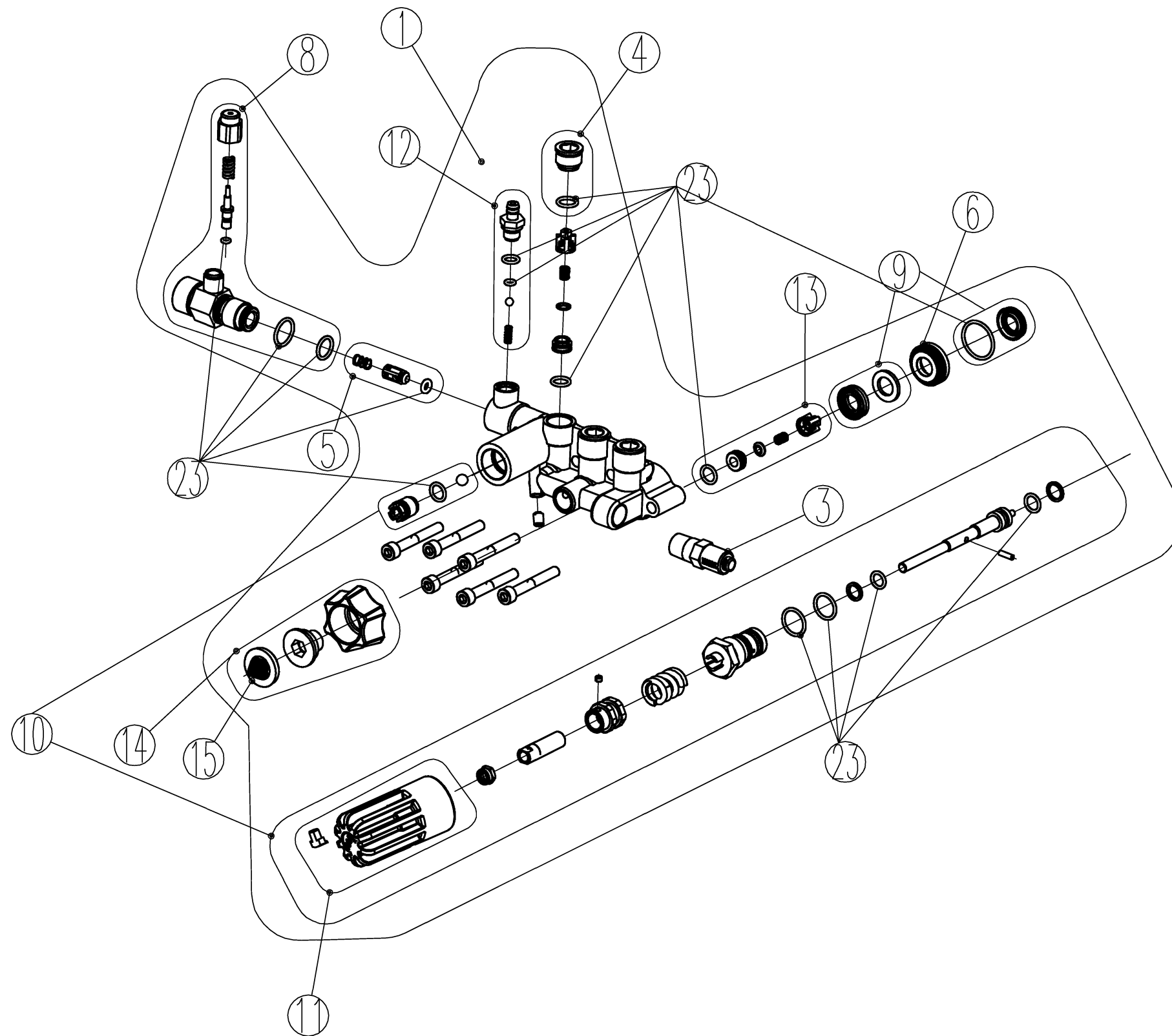
530016 manifold drawing
