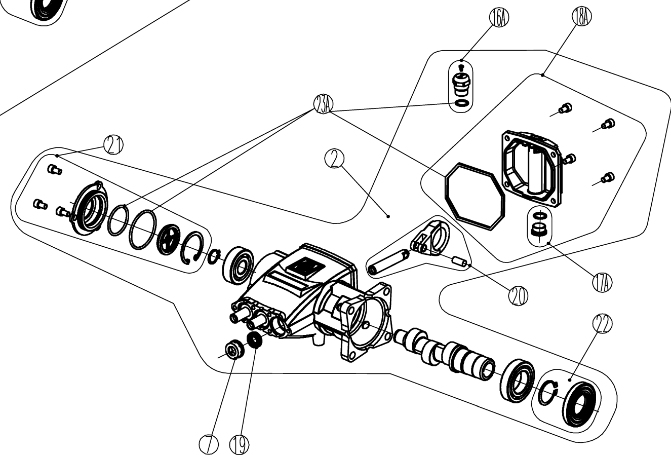
530016 smooth crankcase drawing
