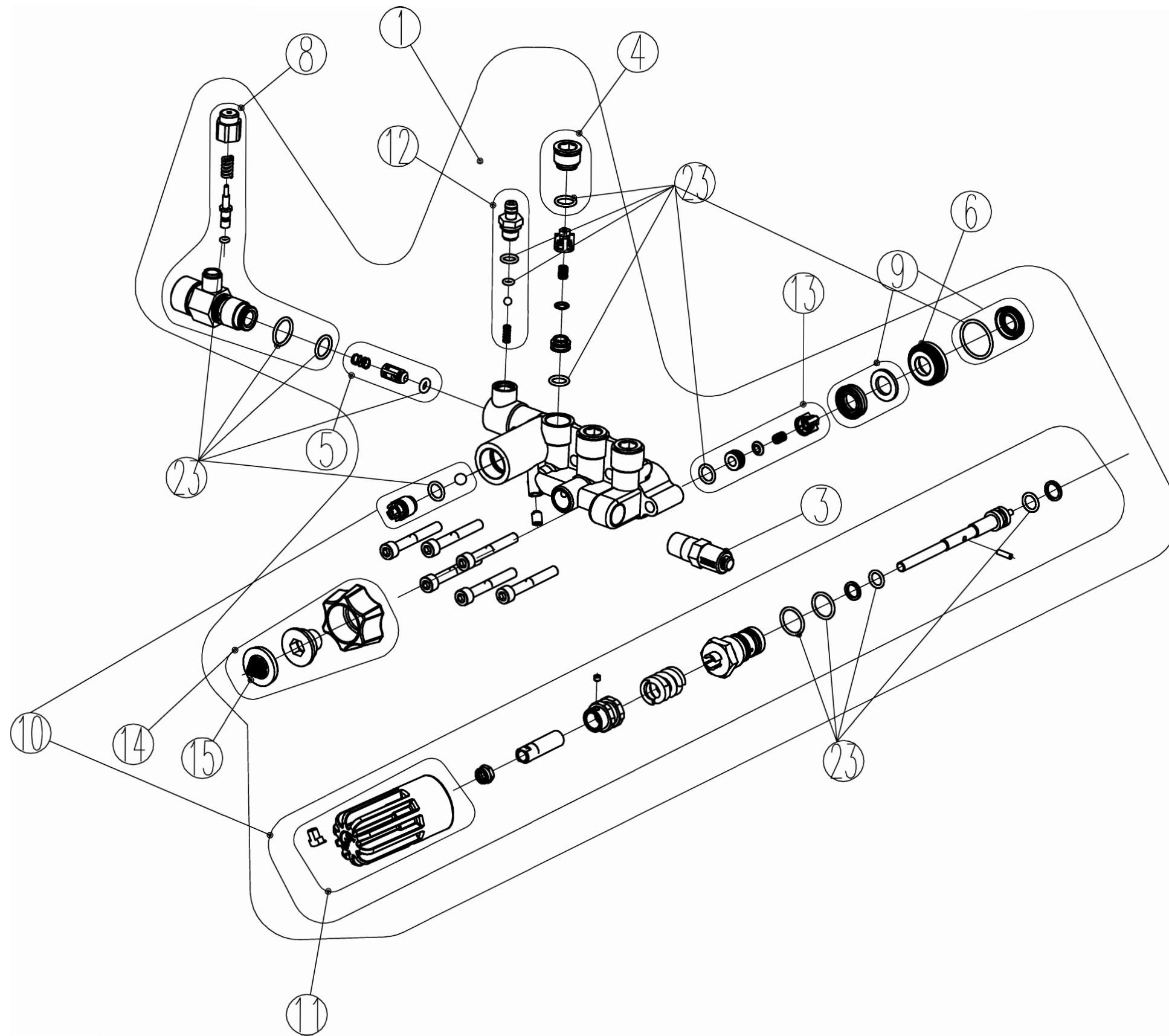
530016 manifold drawing
