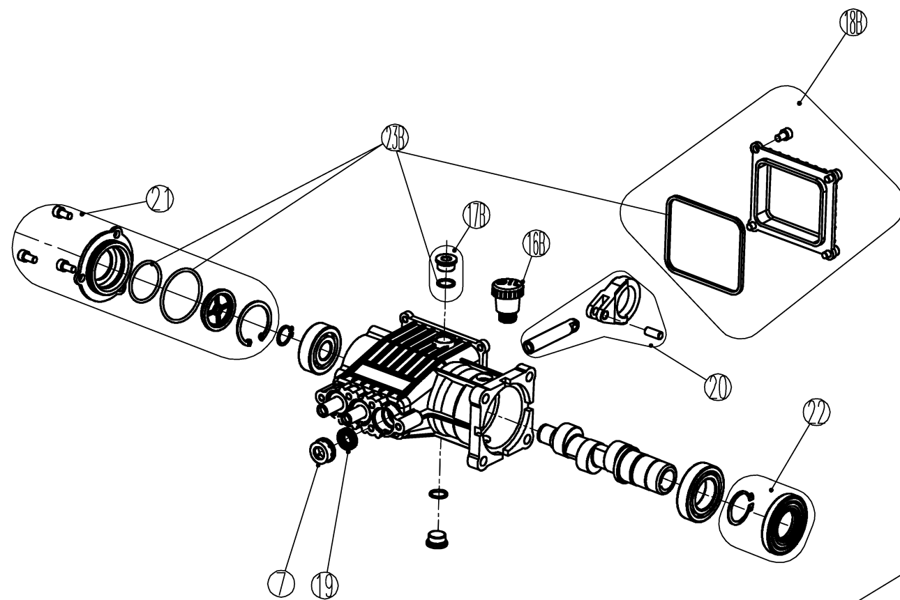
530016 ribbed crankcase drawing
