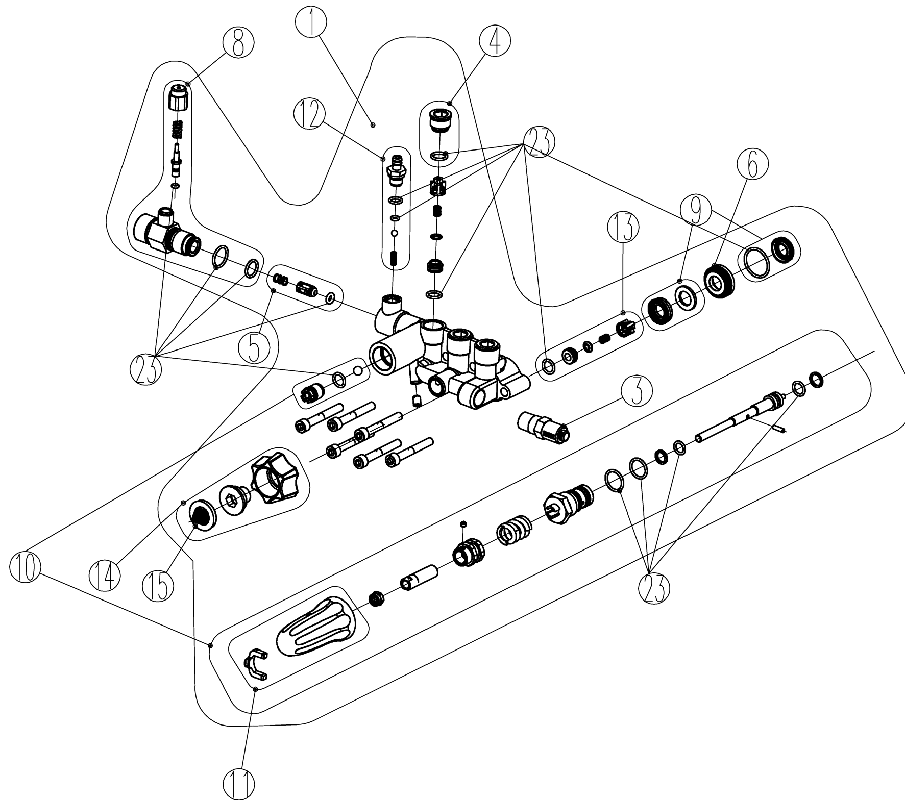
530016 manifold drawing
