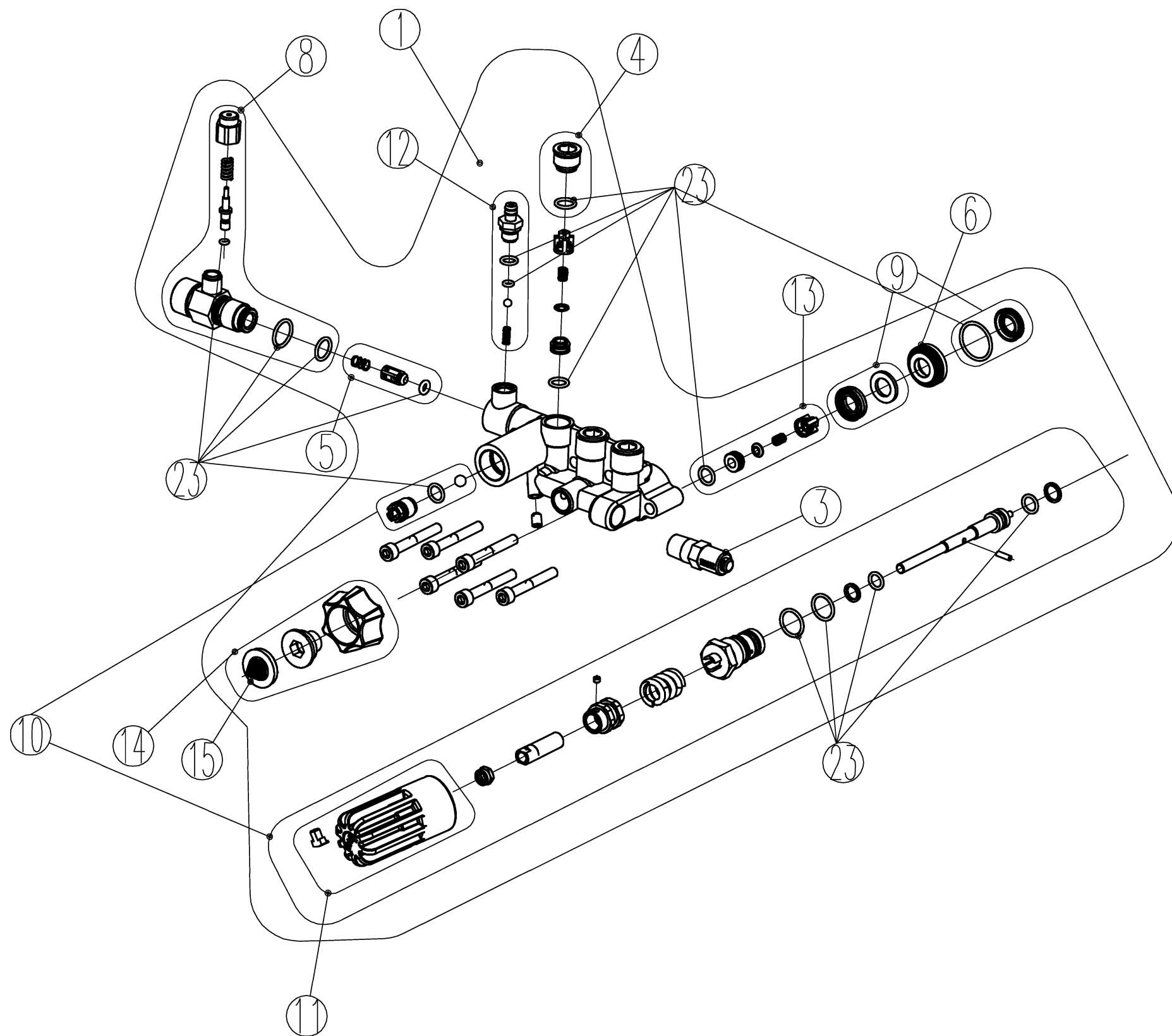
530009 manifold drawing
