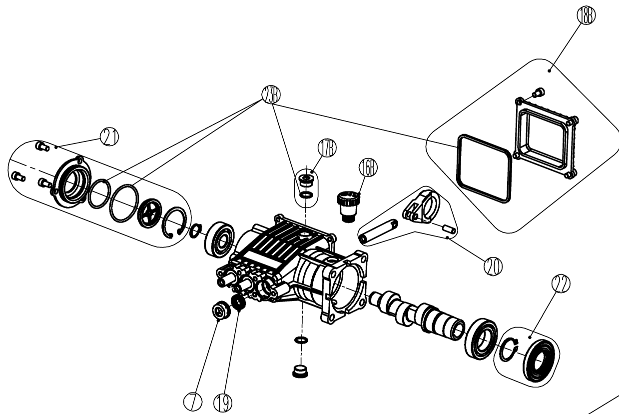
530009 ribbed crankcase drawing
