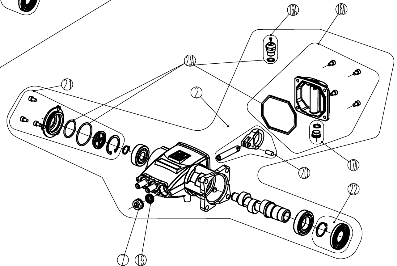
530009 smooth crankcase drawing
