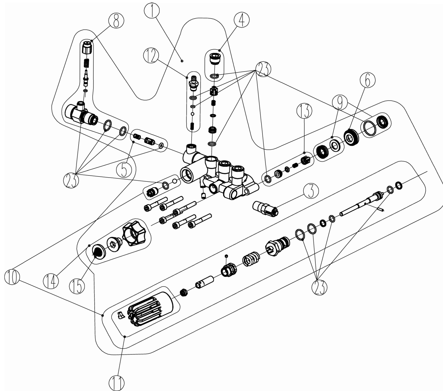
530008 manifold drawing
