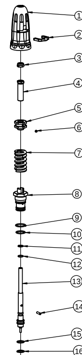
26 PART NO. 7109058 UNLOADER KIT
