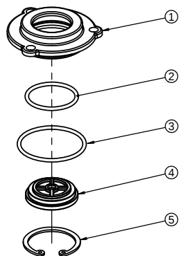
28 PART NO. 7106709 CRANKCASE SIGHTGLASS KIT
