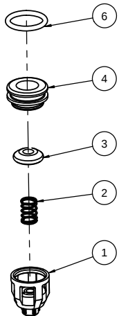
1 PART NO. 7108750 VALVE KIT
