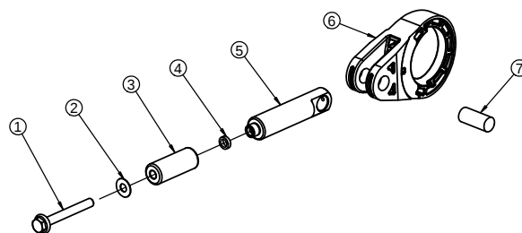
32 PART NO. 7109061 CONNECTING ROD KIT
