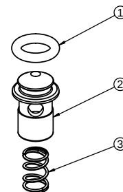
8 PART NO. 7109054 UNLOADER CHECK VALVE KIT
