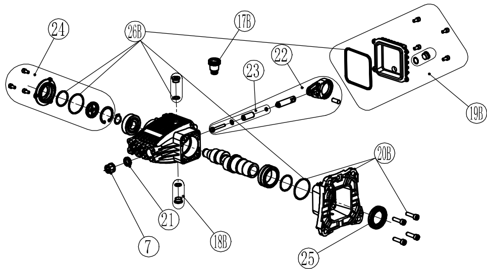
530006 ribbed crankcase drawing
