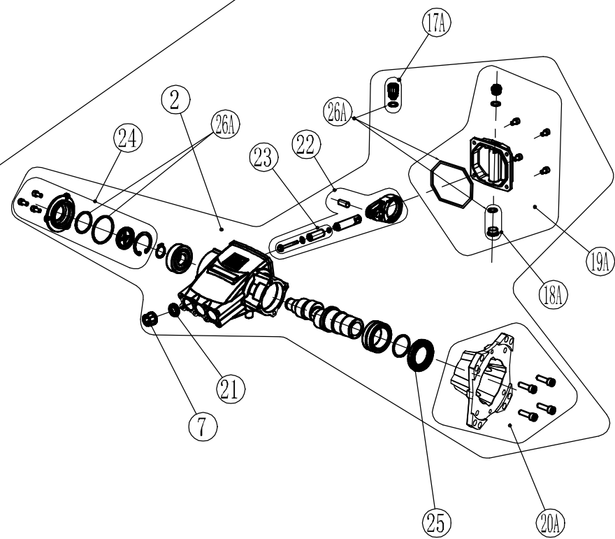
530006 smooth crankcase drawing
