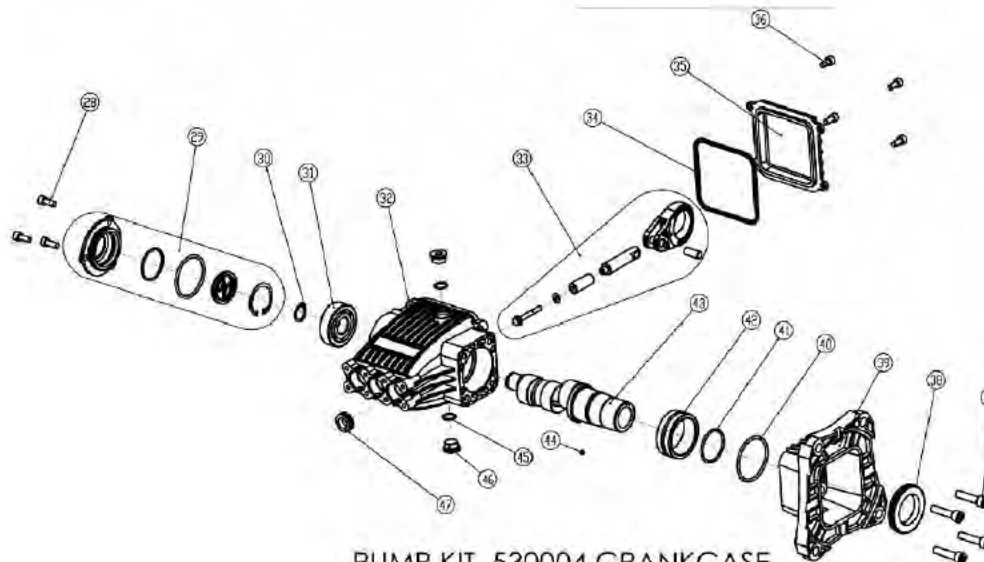
PUMP KIT, 530004 CRANKCASE PART NO. 7107347
