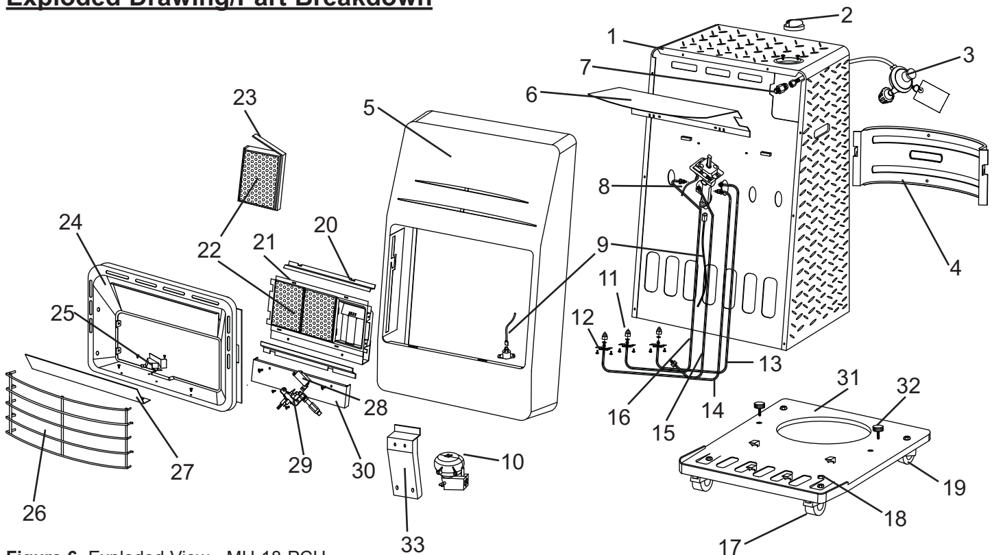
Figure 6. Exploded View - MH-18-PCH
