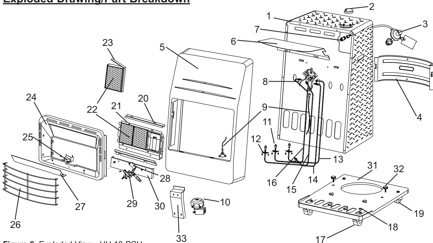
Figure 6. Exploded View - HH-18-PCH
