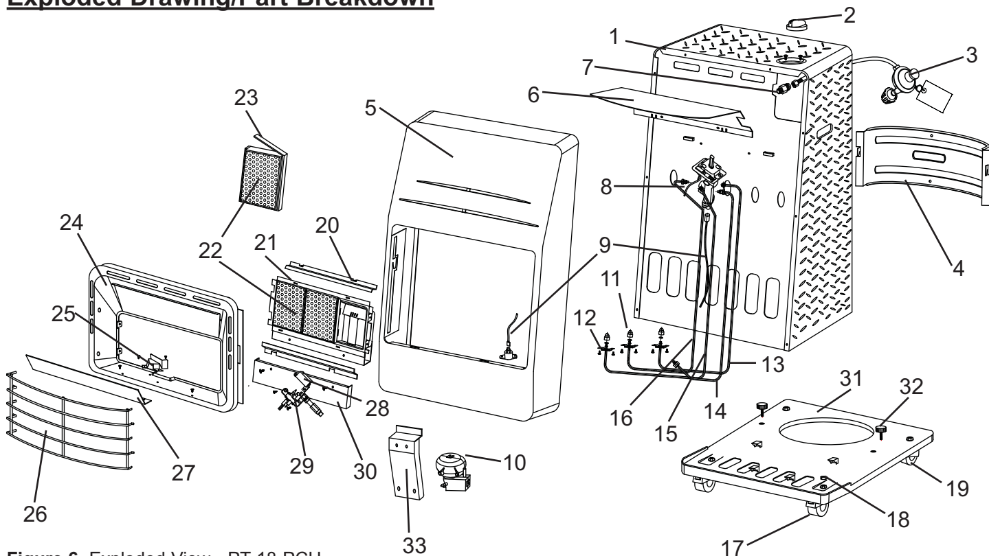
Figure 6. Exploded View - PT-18-PCH
