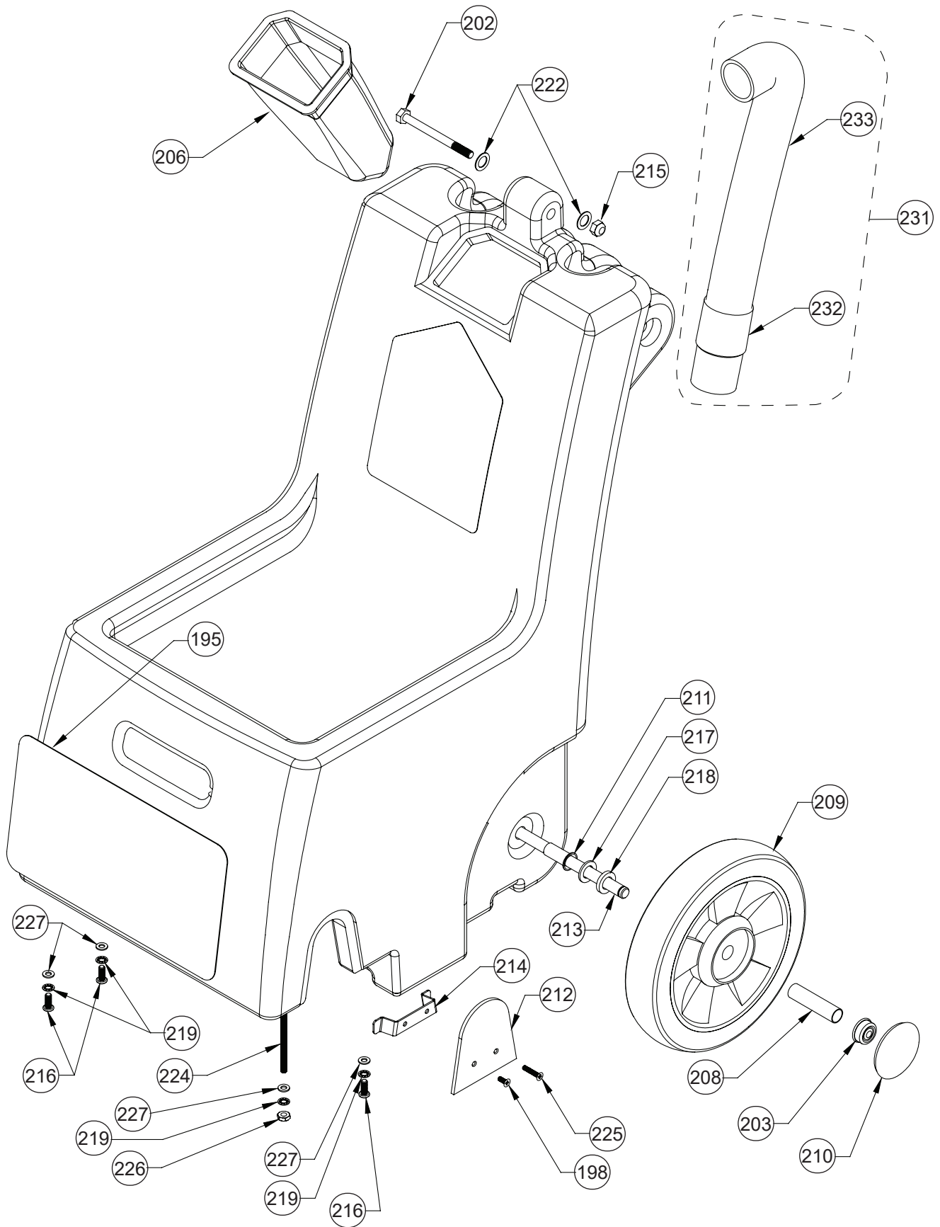
Final Assembly C4-A
