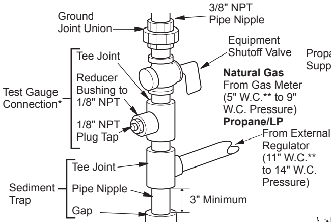
Figure 13 - Gas Connection
