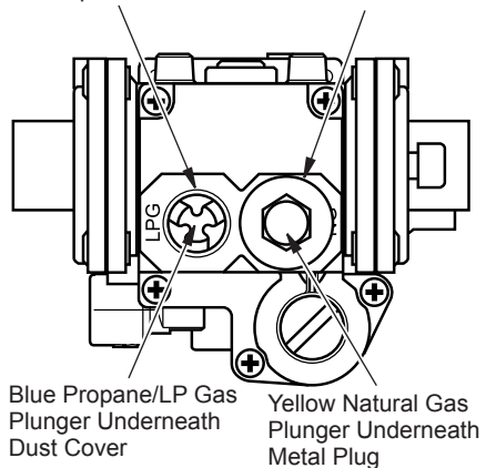
Figure 10 - Gas Regulator
