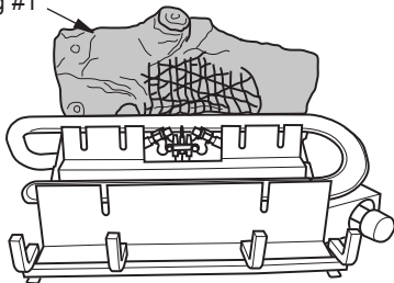
Figure 19 - Installing Log #1
