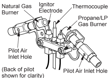
Figure 35 - Pilot Inlet Air Hole
