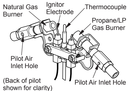
Figure 29 - Pilot
