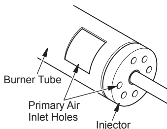
Figure 34 - Burner and Injector Holder
