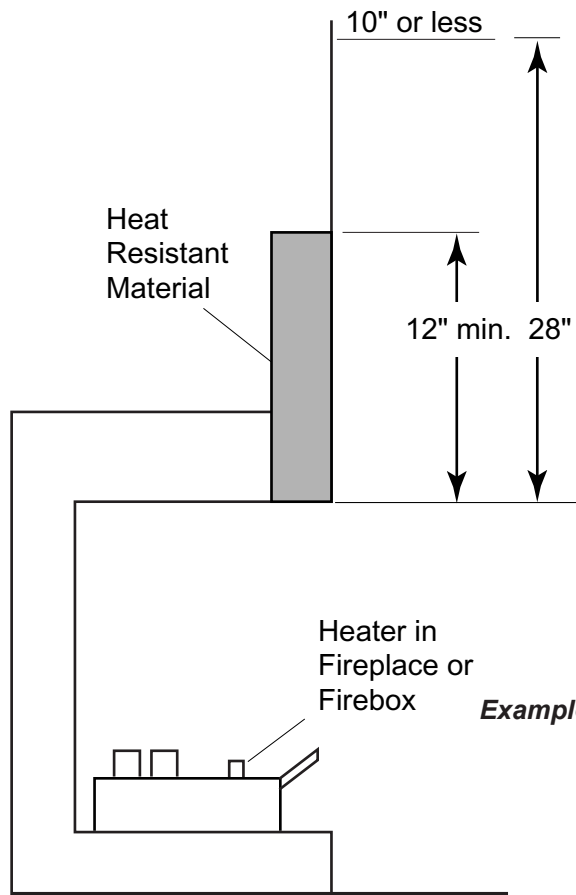
Figure 9 - Minimum Mantel Clearance with No Hood — 24/30TPB
