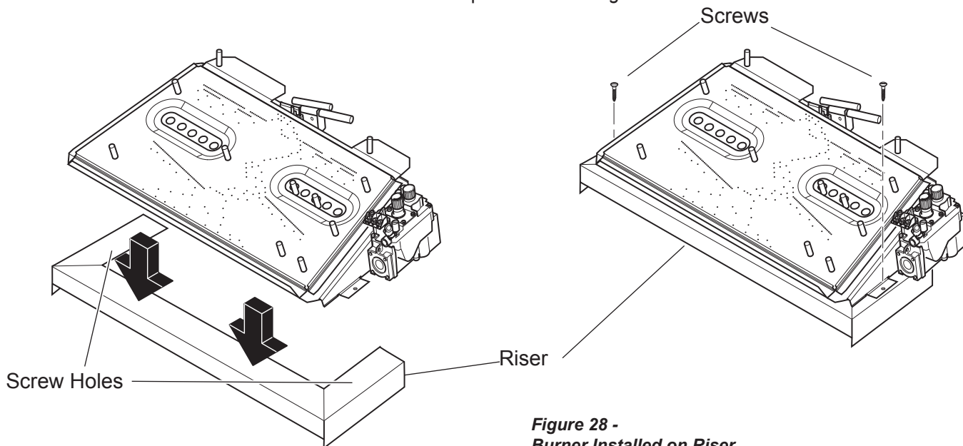
Figure 27 - Placing Burner on Riser
