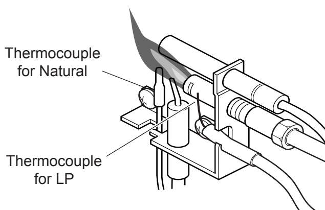
Figure 33 - Correct Appearance of Pilot Flame
