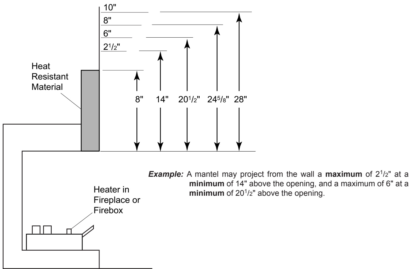
Figure 7 - Minimum Mantel Clearance with No Hood -18TPB
