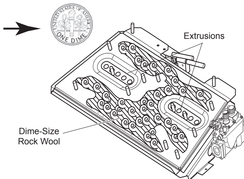
Figure 26 - Placing Rock Wool
