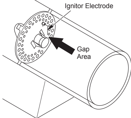
Figure 14 - Clearance Between Ignitor Electrode and Target Plate
