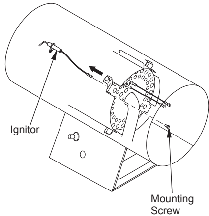
Figure 13 - Removing Ignitor Mounting Screw and Ignitor
