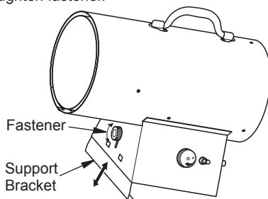
Figure 6 - Adjusting Heater Height Model PCFA60V(-C)
