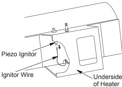
Figure 12 - Removing Ignitor Wire from Piezo Ignitor
