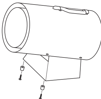
Figure 5 - Attaching Base Feet Model PCFA40(-C)
