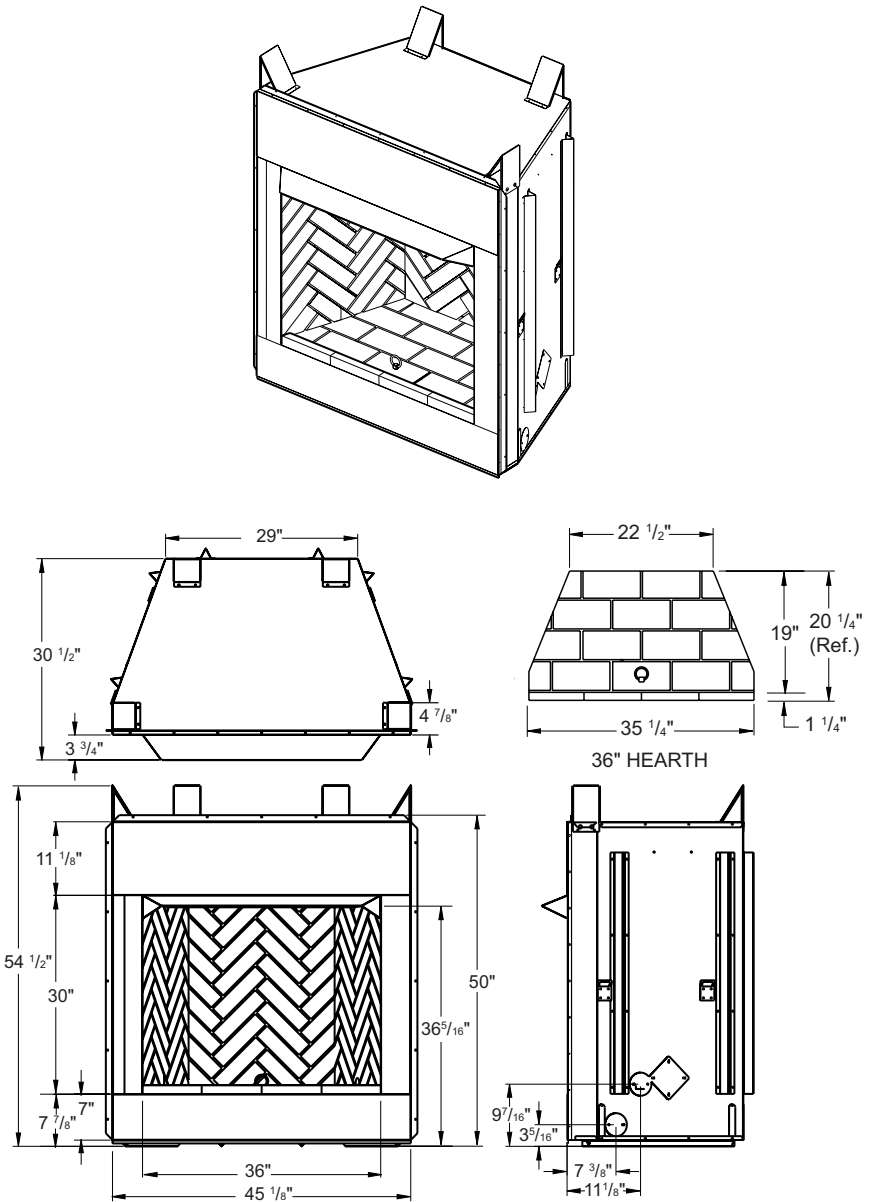
Figure 1 - 36" Models (V)UM36(H,S)(I,R)A and (V)QM36 (H,S)(I,R)A Series
