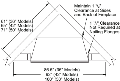
Figure 9 - Corner Installation
