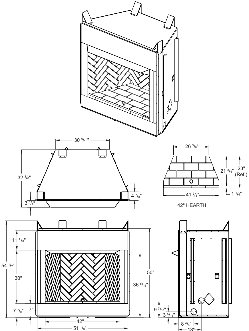
Figure 2 - 42" Models (V)UM42 (H,S)(I,R)A and (V)QM42 (H,S)(I,R)A Series
