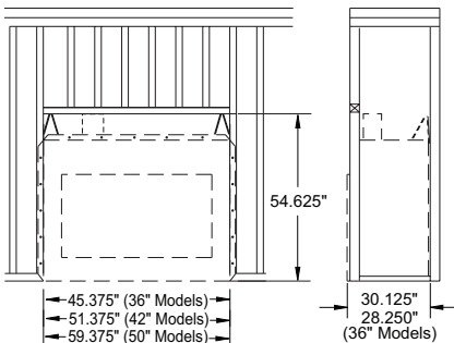
Figure 8 - Framing Dimensions
