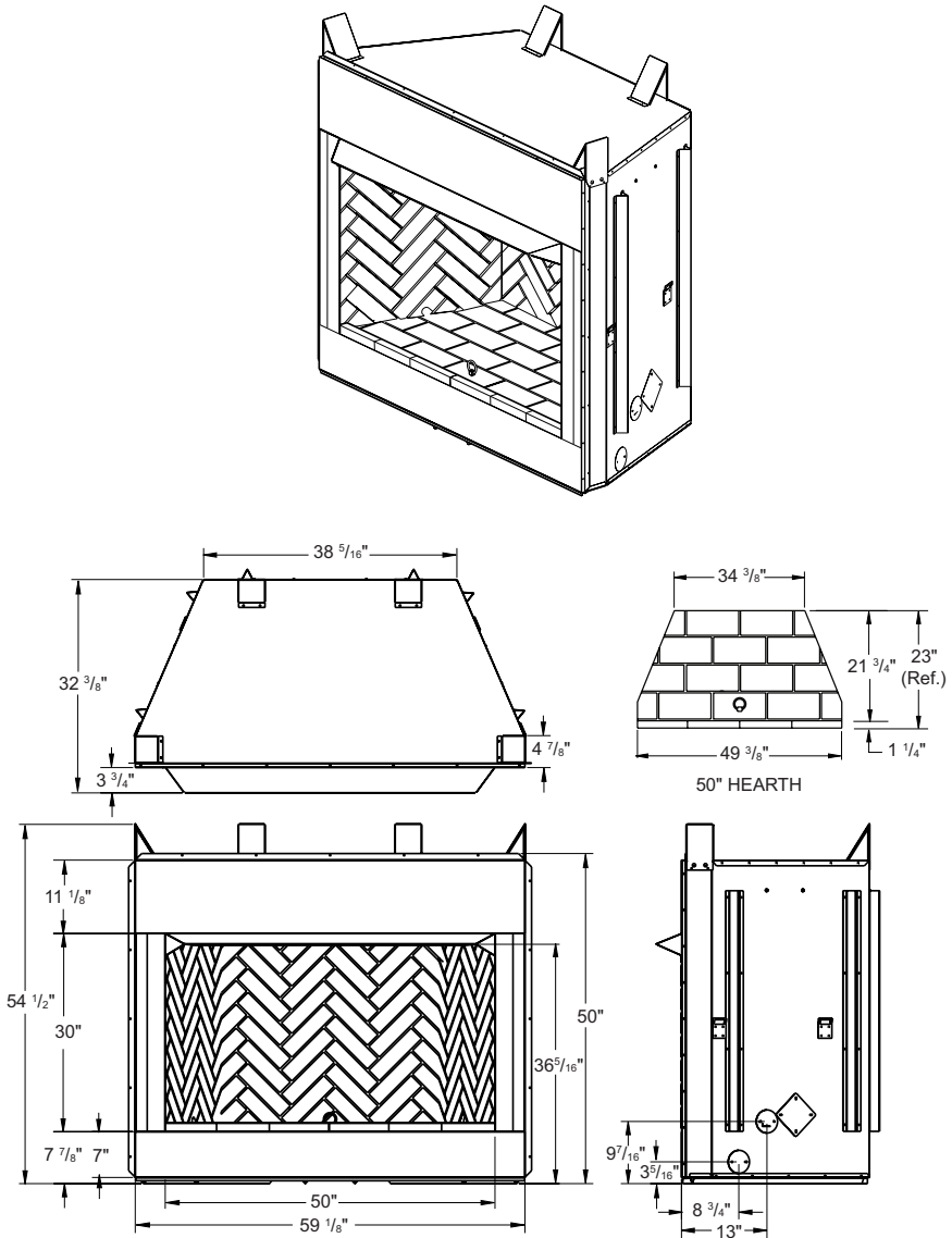
Figure 3 - 50" Models VCM-50(Q,U)A Series
