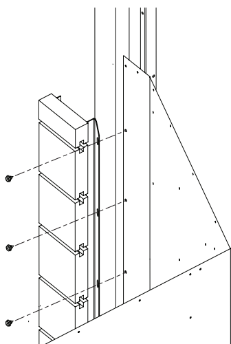
Figure 13 - Installing Leading Bricks
