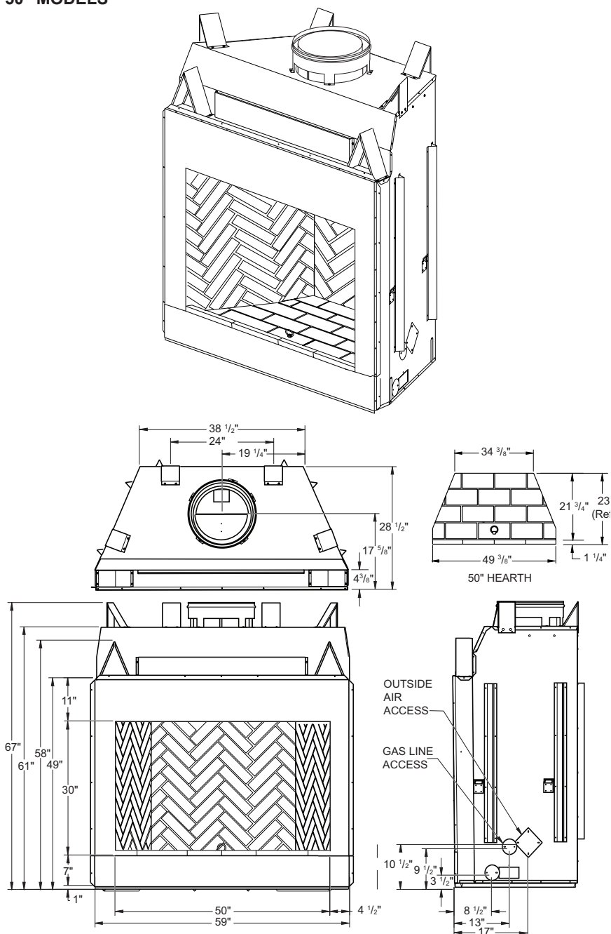
Figure 3 - 50" Models (V)GM50(H,S)(I,R)A AND (V)JM50(H,S)(I,R)A Series
