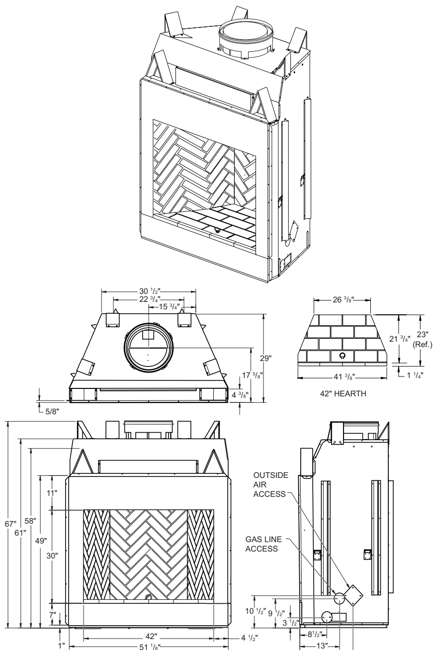
Figure 2 - 42" Models (V)GM42(H,S)(I,R)A AND (V)JM42(H,S)(I,R)A Series
