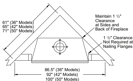
Figure 7 - Corner Installation
