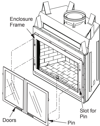
Figure 34 - Installing Glass Doors
