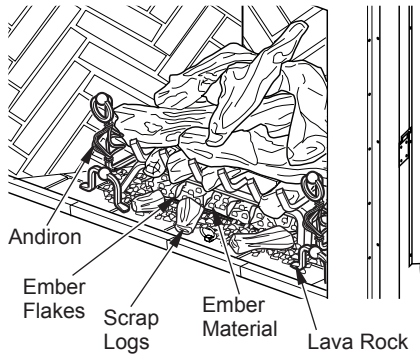
Figure 33 - Installing Floor Media
