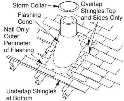
Figure 17 - Flashing Installation
