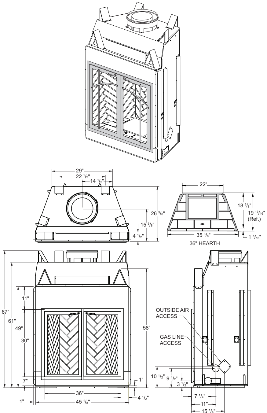
Figure 3 - 36" Model IBVC-36Y
