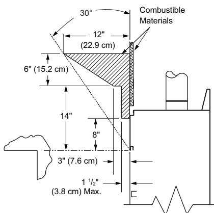
Figure 9 - Mantel Clearances - Side View (Cross Section)
