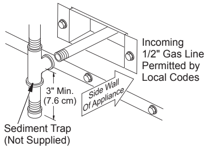
Figure 24 - Sediment Trap
