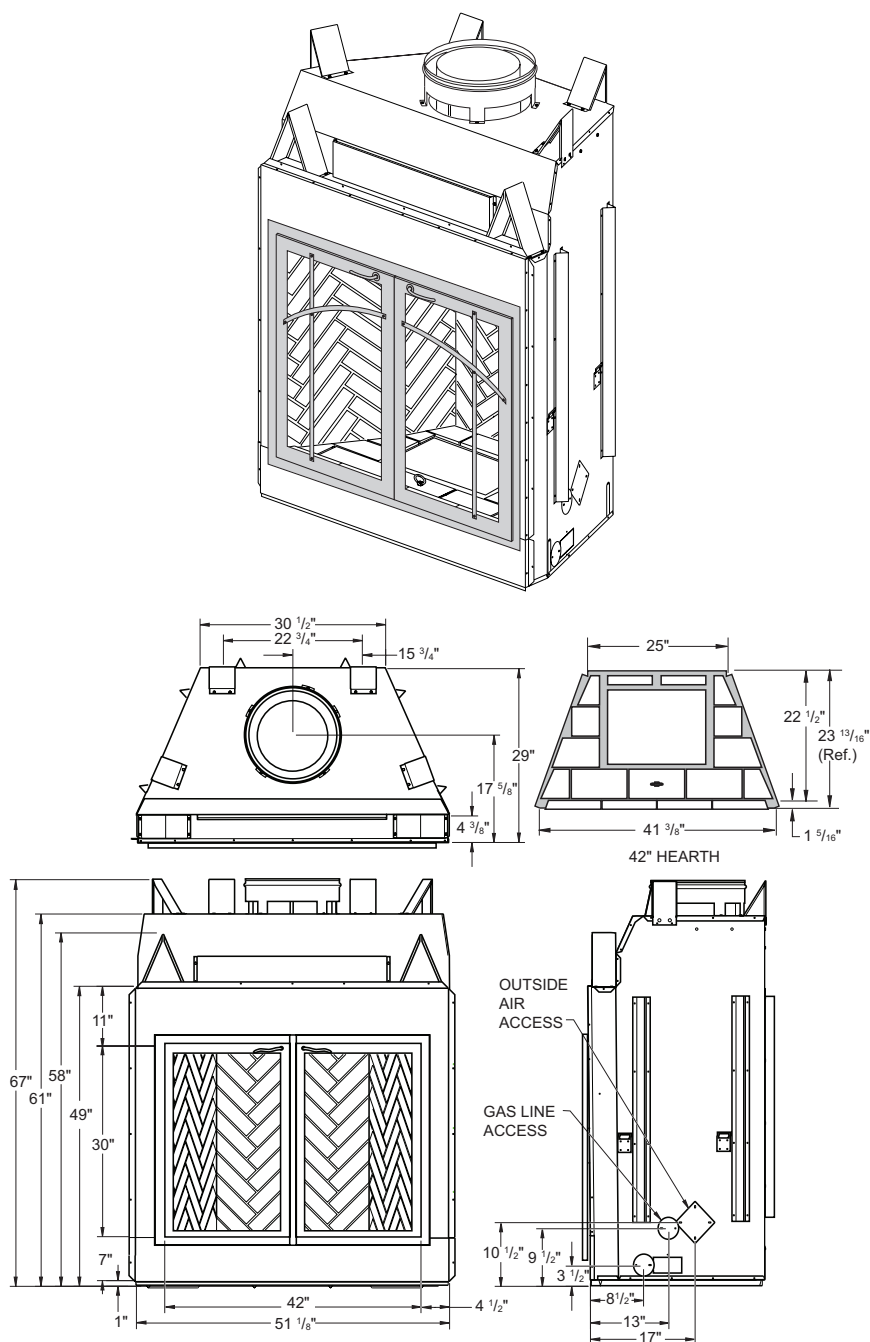
Figure 4 - 42" Model IBVC-42Y
