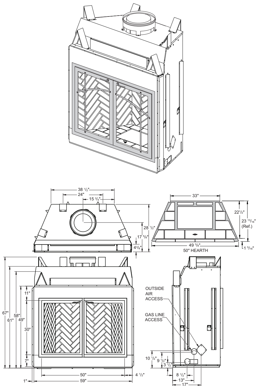
Figure 5 - 50" Model IBVC-50Y
