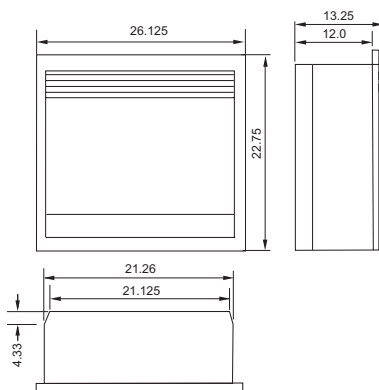
Figure 1 - Heater Dimensions
