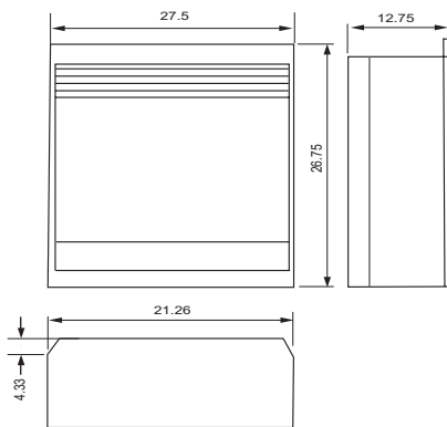
Figure 1 - Heater Dimensions
