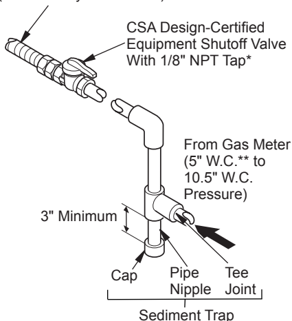
Figure 4 - Gas Connection
