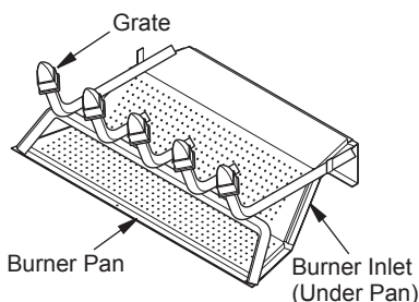
Figure 1 - Product Identification (Ramp Pan Burner)
