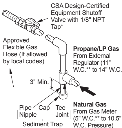
Figure 7 - Gas Connection
