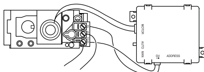
ON/OFF-HI/LO REMOTE MODELS ONLY
