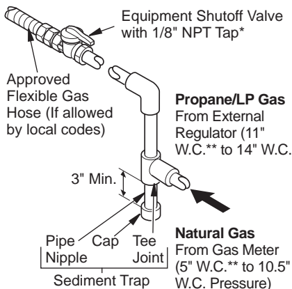
Figure 4 - Gas Connection
