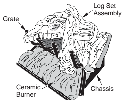
Figure 1 - Product Identification (Ramp Pan Burner)
