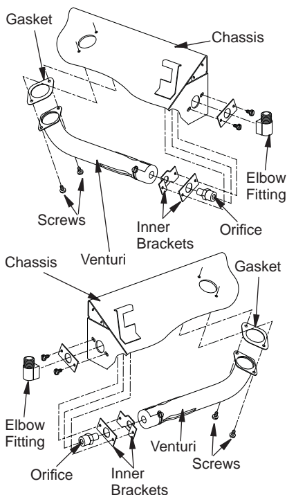
Figure 8 - Repositioning Gas Inlet to Left Side of Unit
