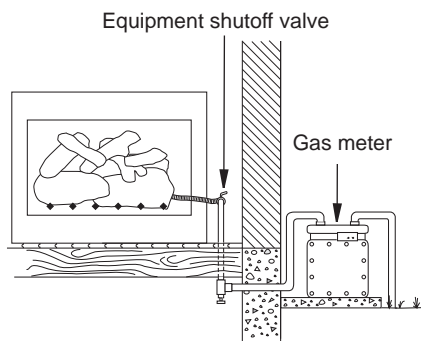
Figure 6 - Checking Gas Joints
