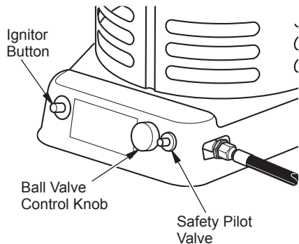
Figure 5 - Starting Heater
