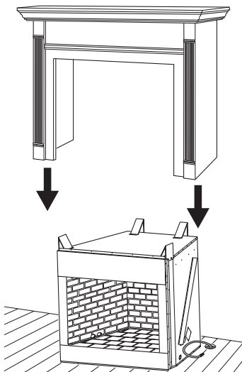
Figure 9 - Inserting Firebox Into Cabinet Mantel (Mantel May Vary From Illustration)
