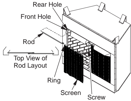
Figure 13 - Installing Fireplace Screen
