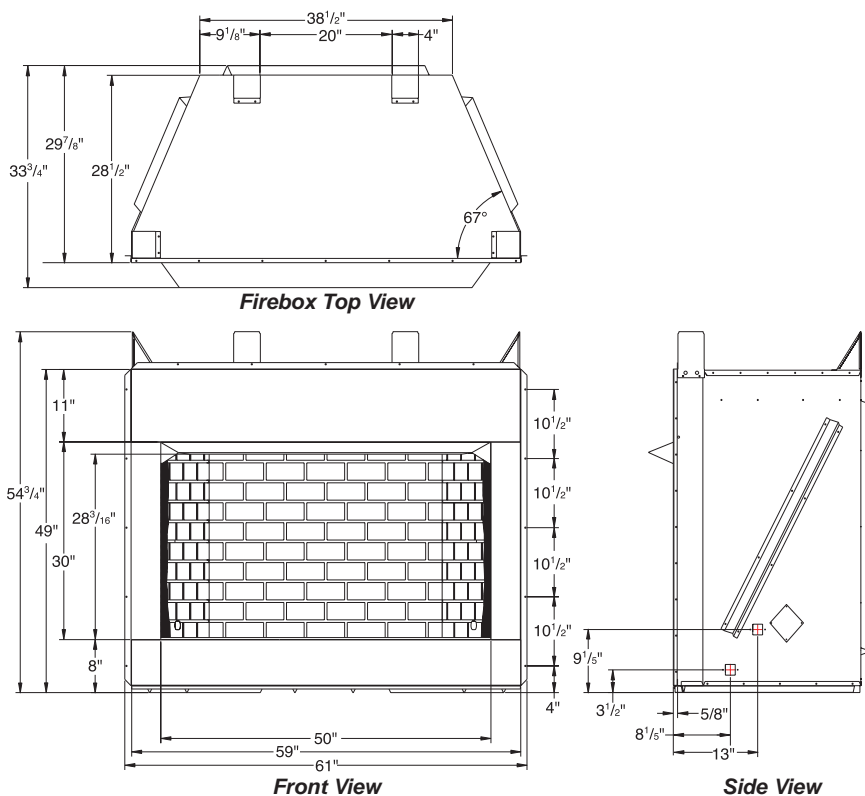
Figure 1 - Firebox Dimensions
