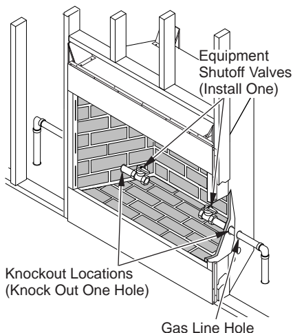
Figure 10 - Installing Gas Line and Equipment Shutoff Valve (Model May Vary From Illustration)
