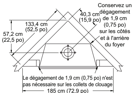
Figure 2 - Installation en coin
