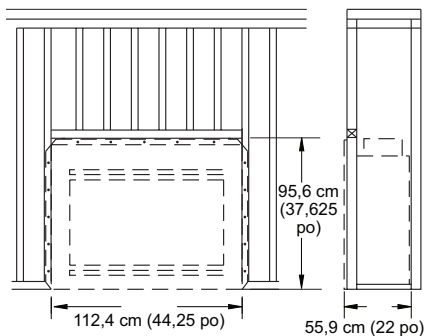
Figure 1 - Dimensions de la structure
