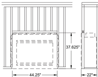
Figure 1 - Framing Dimensions
