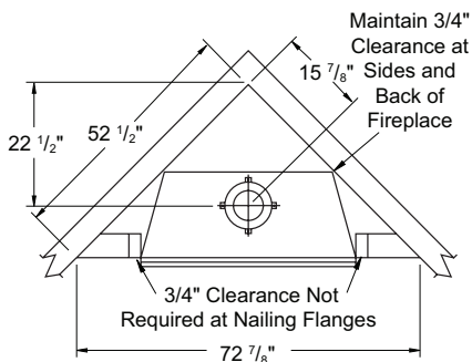
Figure 2 - Corner Installation
