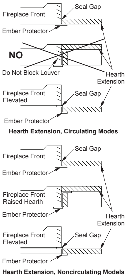
Figure 3 - Hearth Extension
