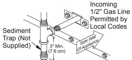
Figure 19 - Sediment Trap
