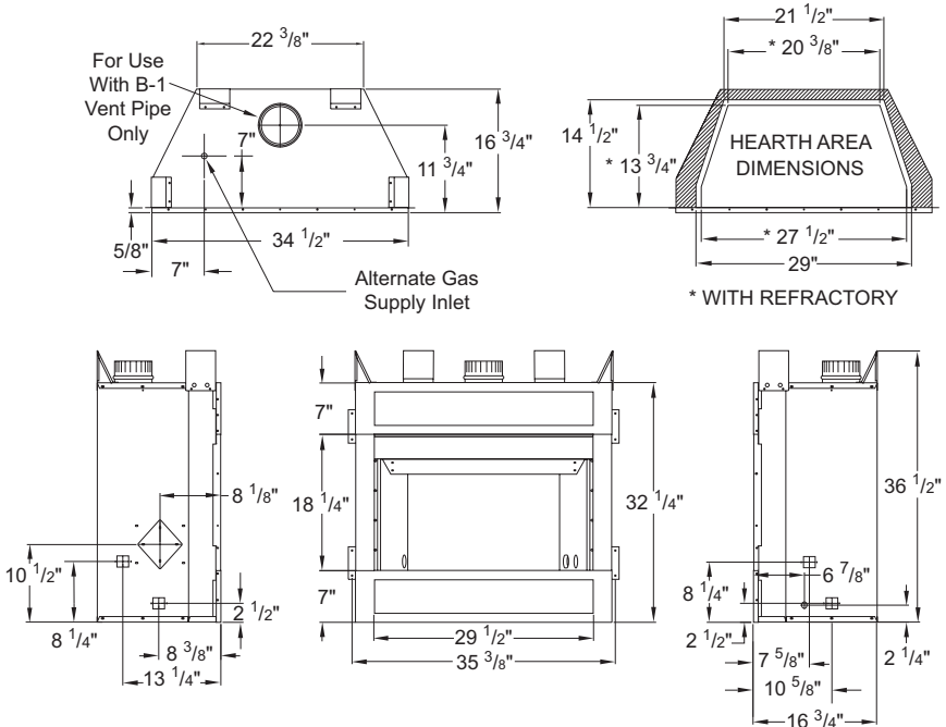
Figure 1 - Appliance Dimensions
