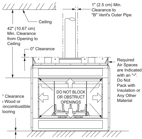
Figure 4 - Minimum Clearances (Front View)
