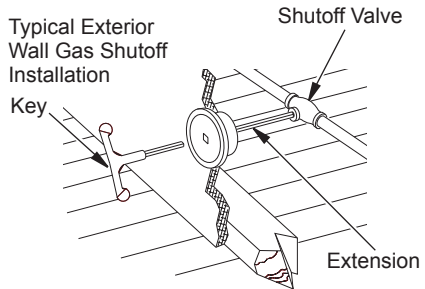
Figure 17 - Manual Shutoff Valve Installation
