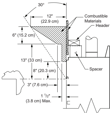
Figure 5 - Mantel Clearances - Side View (Cross Section)
