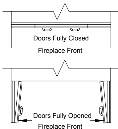
Figure 24 - Glass Doors
