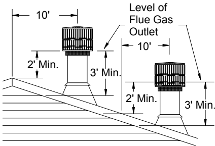
Figure 20 - 10 Foot Rule
