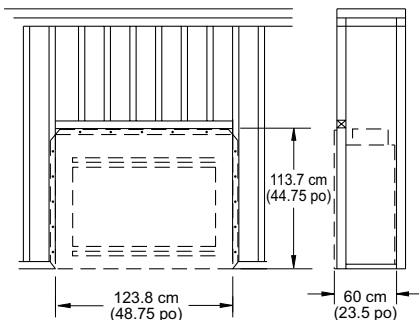
Figure 1 - Dimensions de la structure
