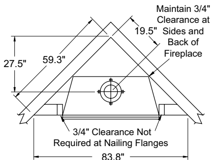
Figure 2 - Corner Installation
