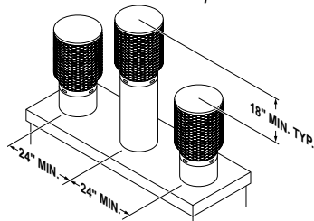
Figure 19 - Multiple Chase Installation
