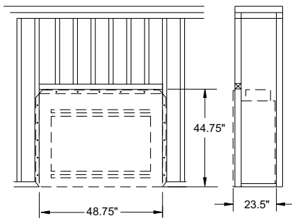
Figure 1 - Framing Dimensions
