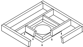
Figure 13 - Firestop Spacer with Living Space Above Ceiling
