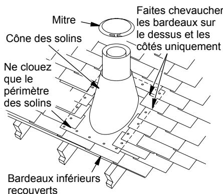
Figure 16 - Installation des solins
