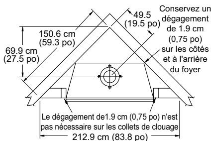
Figure 2 - Installation en coin
