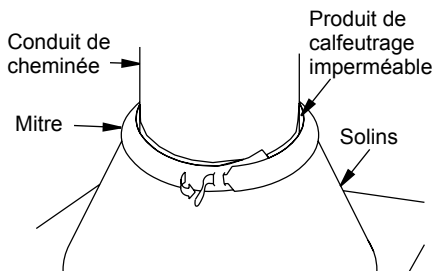
Figure 17 - Mitrer
