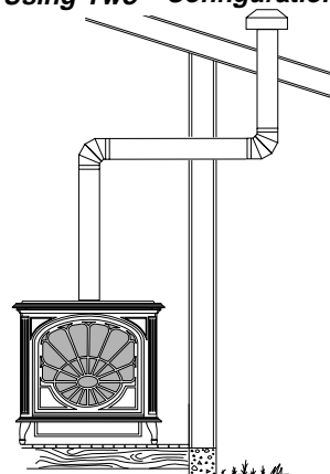
Figure 24 - Venting Through a Side Wall
