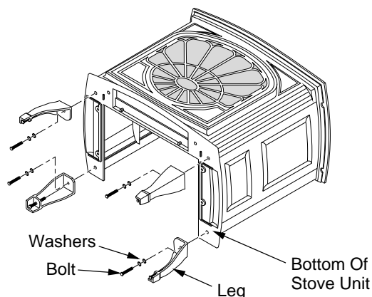
Figure 10 - Attaching Stove Legs
