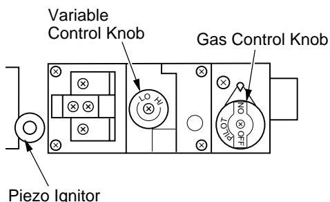
Figure 48 - Control Valve
