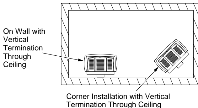
Figure 2 - Common Stove Locations
