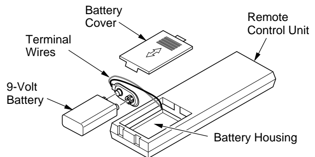
Figure 39 - Installing Battery in Hand-Held Remote Control Unit (GHRC Only)
