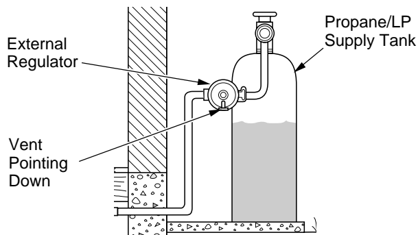
Figure 28 - External Regulator with Vent Pointing Down (Propane/LP Only)
