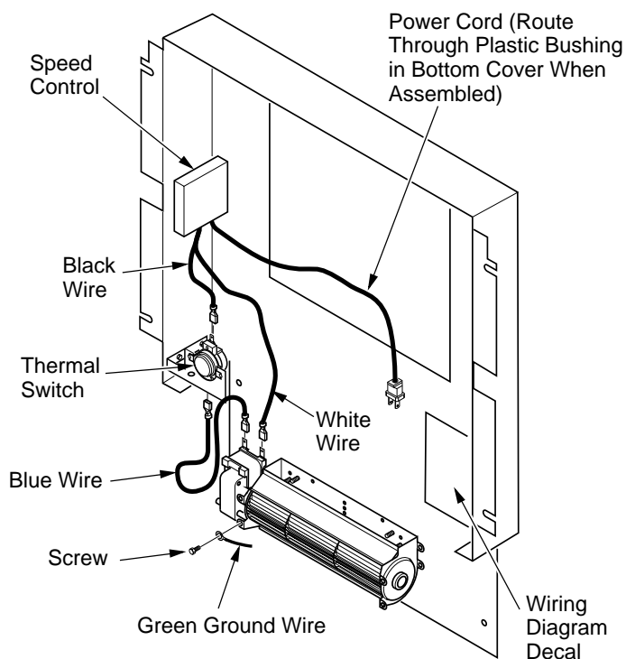
Figure 18 - Blower Wiring Layout
