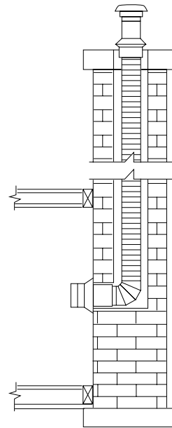
Figure 26 - Straight Installation into Masonry Chimney
