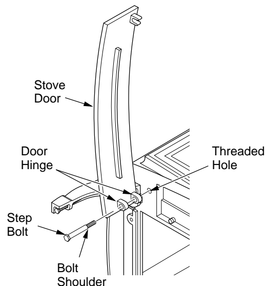
Figure 11 - Attaching Stove Door
