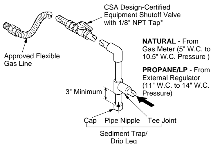
Figure 29 - Gas Connection
