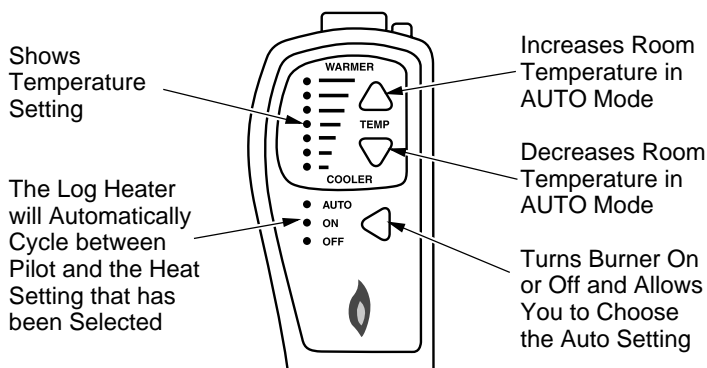
Figure 50 - Hand-Held Thermostat Remote Control Unit Selections (GHRCTA Only)
