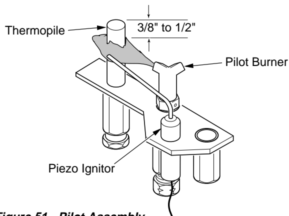
Figure 51 - Pilot Assembly
