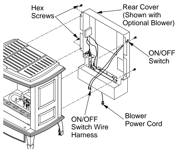
Figure 19 - Installing Rear Cover (Shown with Optional Blower Accessory)
