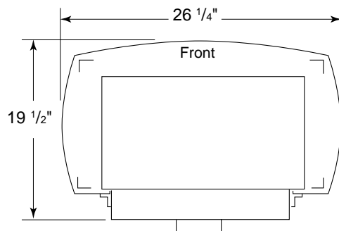
Figure 5 - Stove With Burner System Bottom Dimensions
