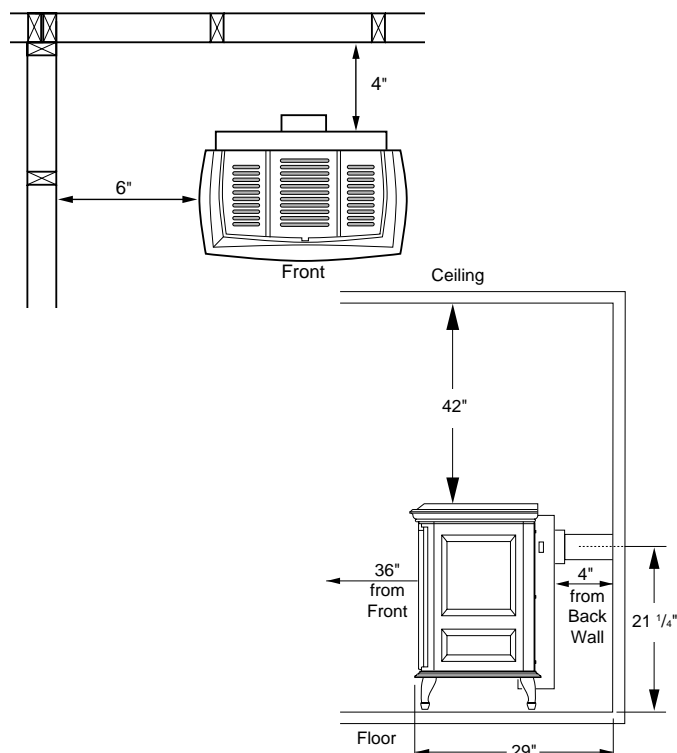
Figure 3 - Clearances for Standard Installation
