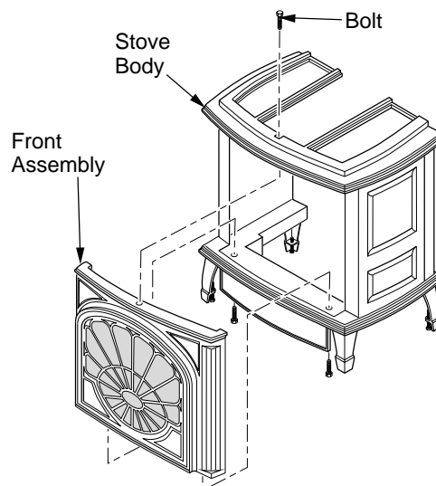
Figure 13 - Removing Front Assembly
