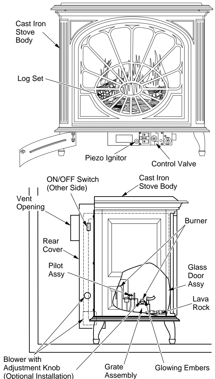
Figure 1 - B-Vent Burner System Shown Installed in Approved DESA International Cast Iron Stove Body Models SCIVFC Series and PSCIVFC Series Only
