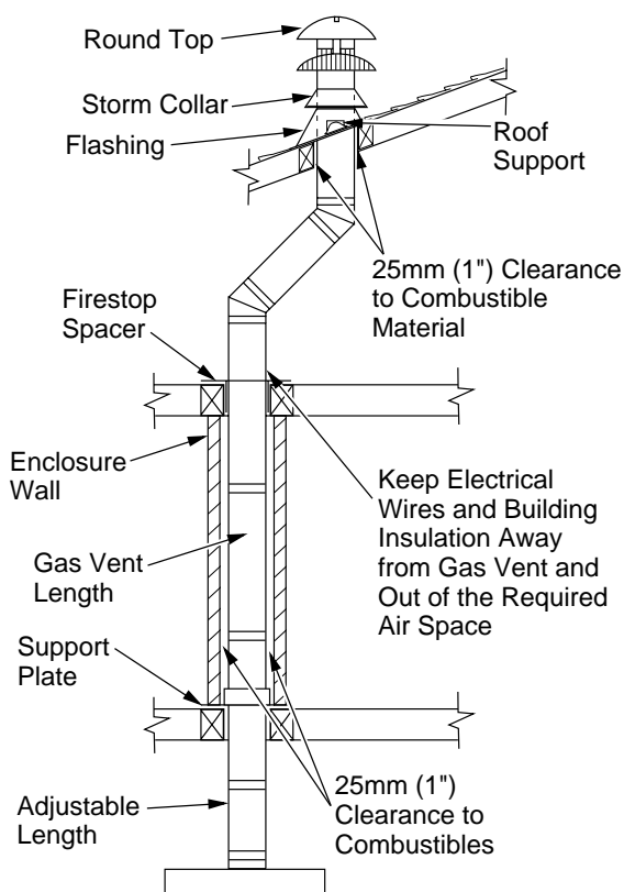
Figure 21 - Typical B-Vent Installation
