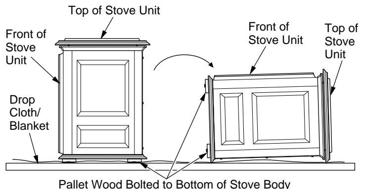
Figure 7 - Laying Down Stove On Side
