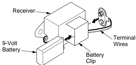
Figure 37 - Installing Battery in Receiver
