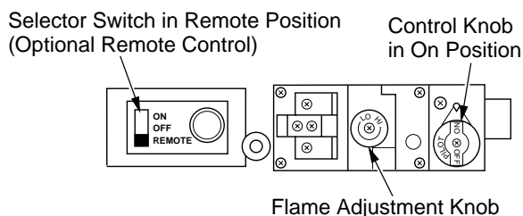
Figure 49 - Setting the Selector Switch, control Knob, and Flame Adjustment Knob for Remote Operation
