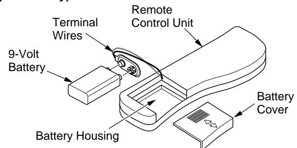
Figure 40 - Installing Battery in Hand-Held Remote Control Unit (GHRCTA Only)
