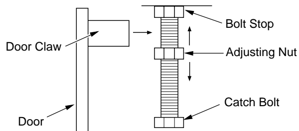
Figure 12 - Catch Bolt and Door Claw Orientation
