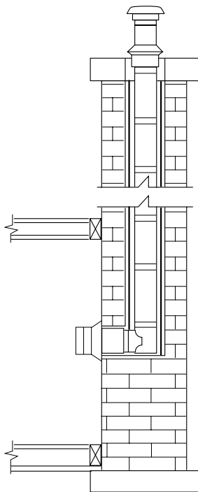
Figure 27 - Typical Straight Installation with Listed Chimney Liner
