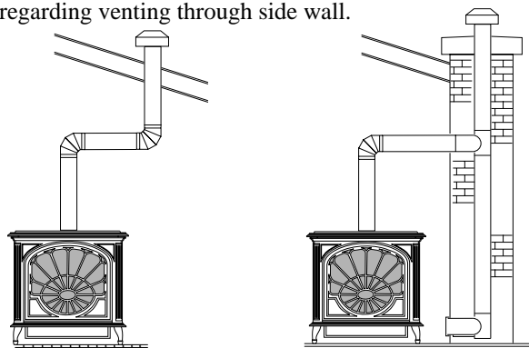
Figure 22 - Vertical Venting Through Ceiling Using Two 90° Elbows
