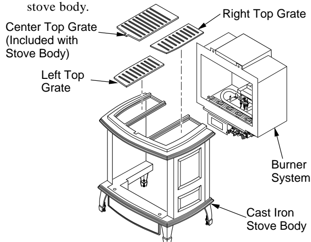
Figure 15 - Installing Burner System Into Cast Iron Stove Body
