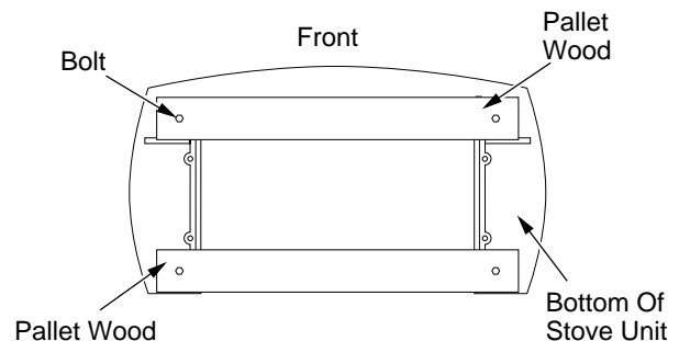
Figure 8 - Removing Pallet Wood From The Bottom of The Stove
