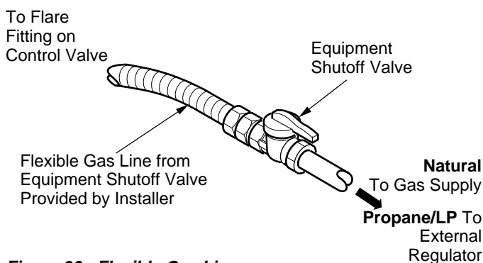
Figure 30 - Flexible Gas Line
