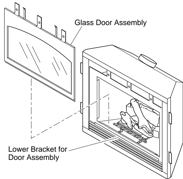
Figure 2 - Removing Glass Door Assembly
