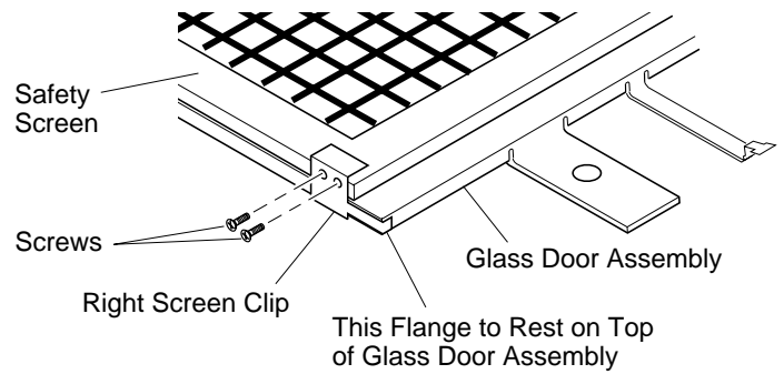
Figure 4 - Attaching Upper Clip to Safety Screen and Glass Door Assembly (Right Side Shown)
