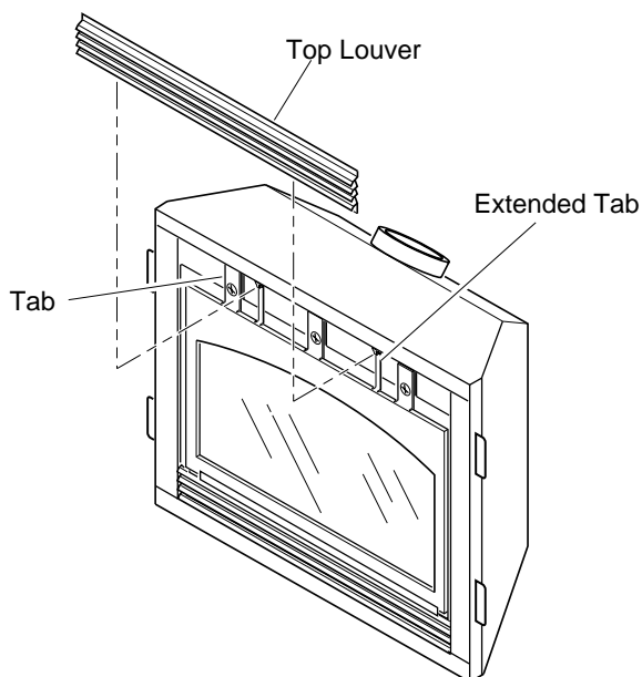
Figure 1 - Removing/Replacing Top Louver
