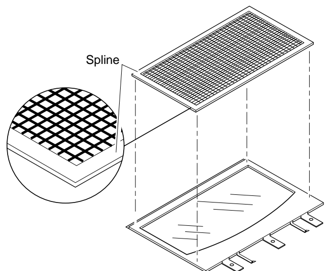
Figure 3 - Placing Safety Screen on Glass Door
