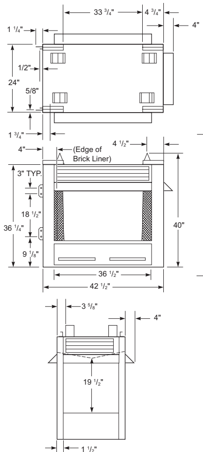
Figure 1 - Peninsula (Three-Sided) Firebox
