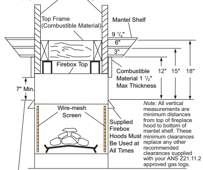
Figure 7 - Minimum Mantel Clearances for Built-In Installation
