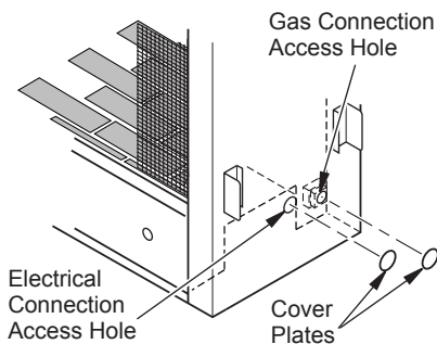
Figure 15 - Locating Electrical Connection and Gas Connection on Either Side of Fireplace
