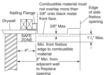
Figure 9 - Framing for Built-In Firebox Installation: Top View
