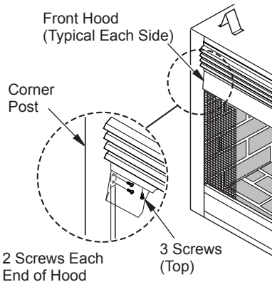
Figure 19 - Typical Hood Installation (Both Sides)
