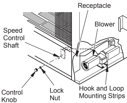
Figure 18 - Installing Optional Blower GA3500A
