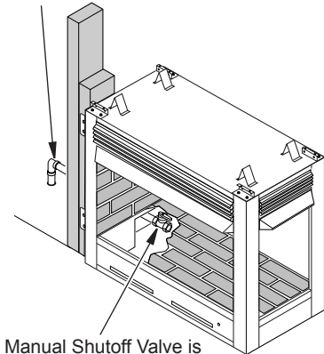
Figure 11 - Installing Gas Line and Manual Shutoff Valve
