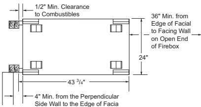
Figure 6 - Minimum Clearance - Top View
