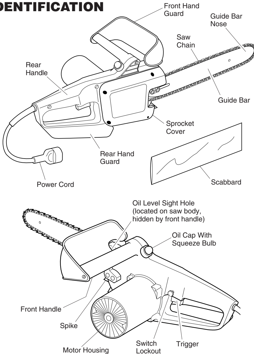
Figure 2 - Electric Chain Saw
