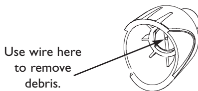
Figure 18 — Nozzle Maintenance
