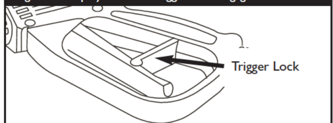
Figure 9 — Spray Gun with Trigger Lock Engaged
