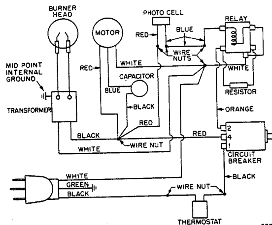
Figure 6. Wiring Diagrams
