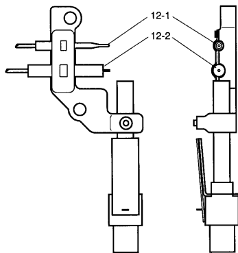
Pilot And Bracket Assembly
